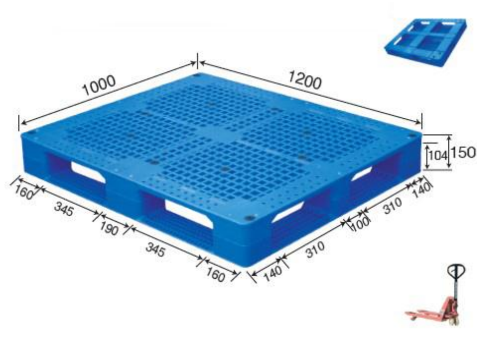
No. 97 MR - 1210E Double Deck (Steel reinforced)
