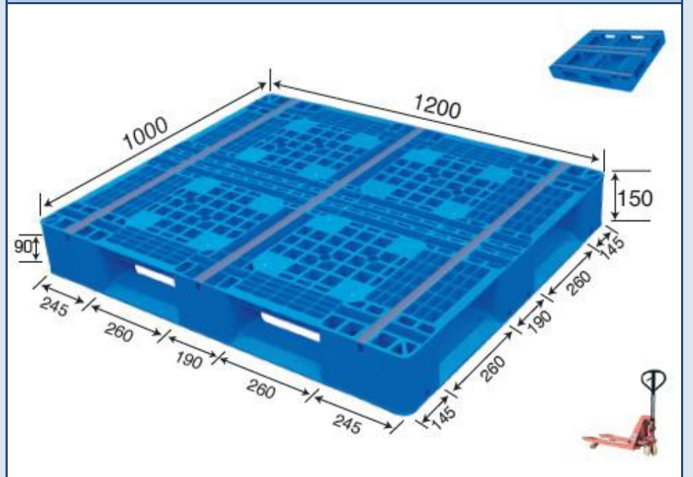
No. 101 MR - 1210D Double Deck (Steel reinforced)
