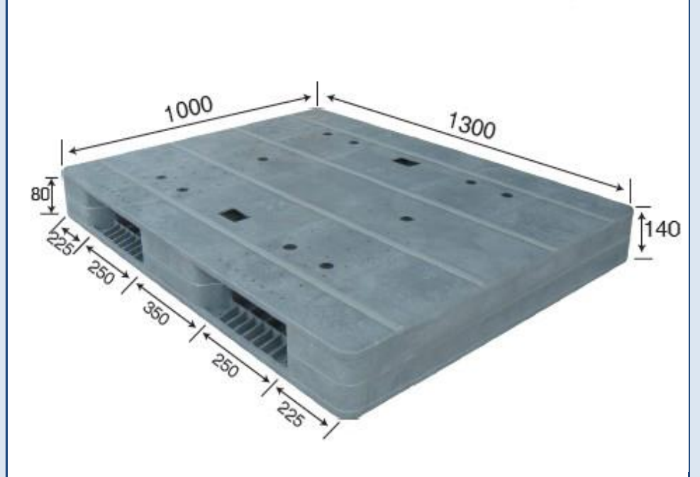
No. 677 MR - 1310 Flat Reversible
