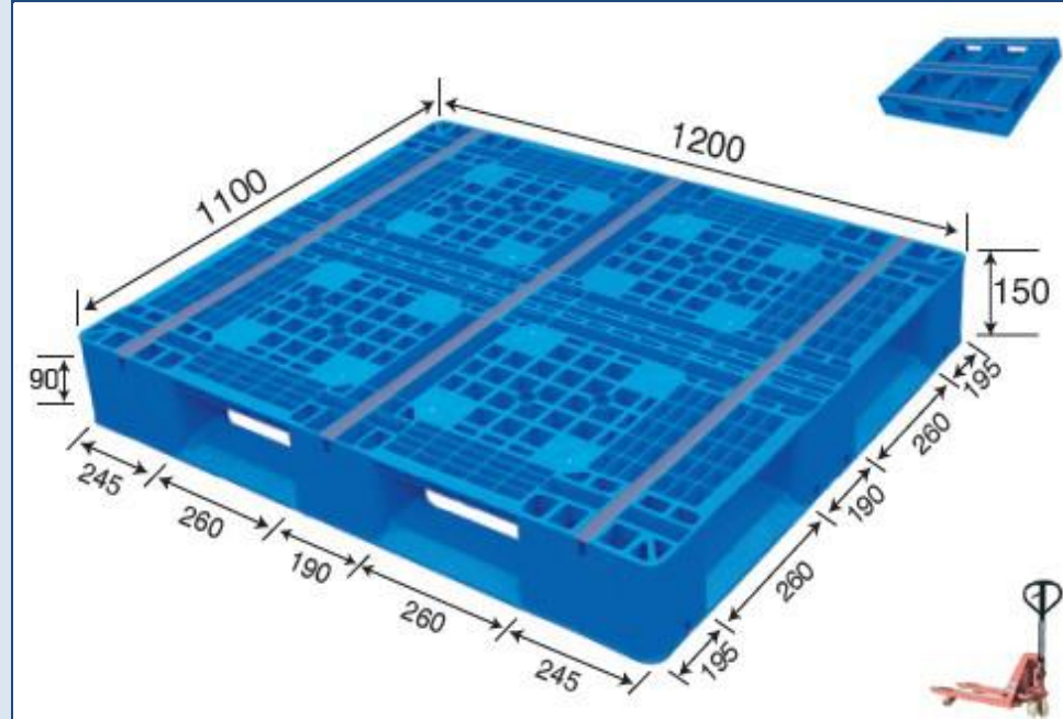
No. 518 MR - 1211D Double Deck (Steel reinforced)
