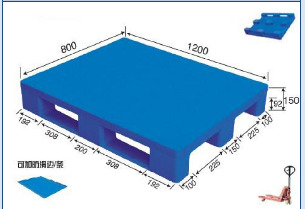
No. 690 MR - 1208 Flat Three Runner
