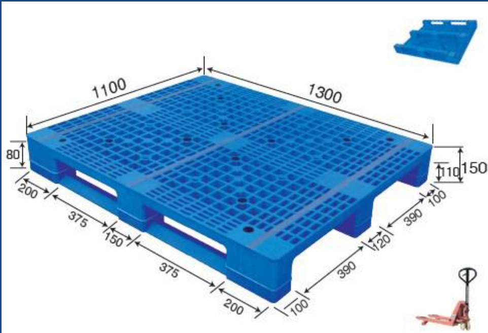
No. 541 MR - 1311 Three Runner (Steel reinforced)
