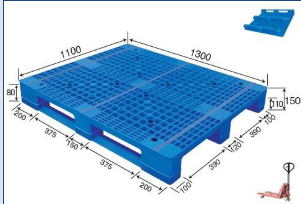
No. 540 MR - 1311 Three Runner (Steel reinforced)
