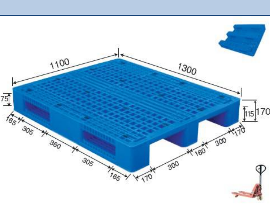
No. 544 MR - 1311B Three Runner
