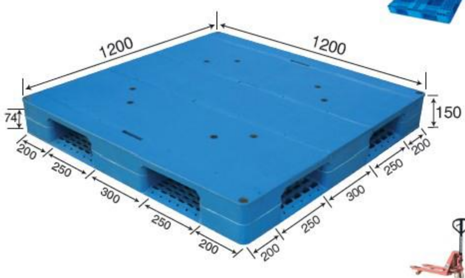
No. 414 MR - 1212D Flat Double Deck (Steel reinforced)
