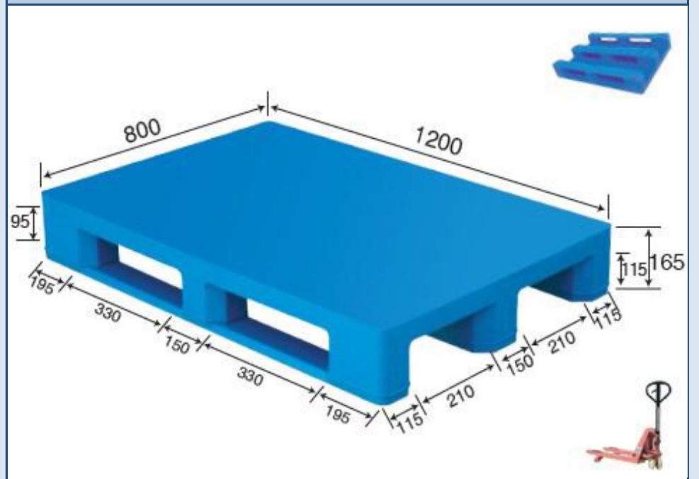
No. 696 MR - 1208 Flat Three Runner
