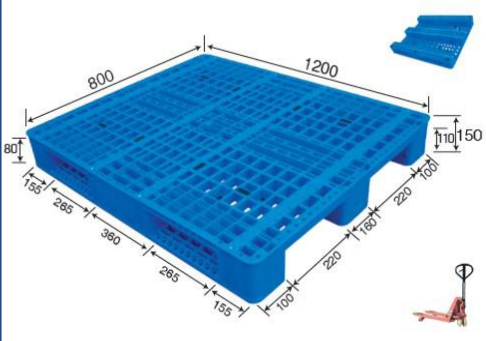
No. 698 MR - 1208D Three Runner (Steel reinforced)
