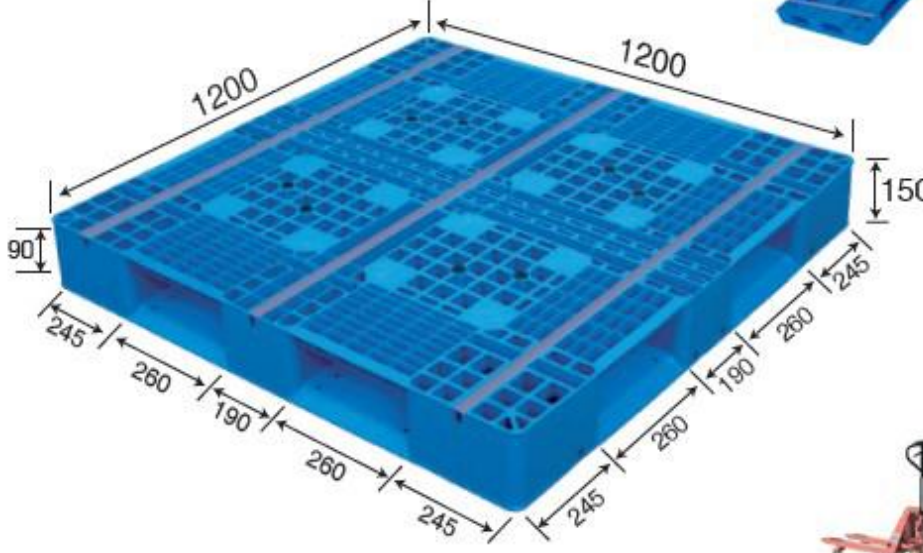
No. 411 MR - 1212D Double Deck (Steel reinforced)
