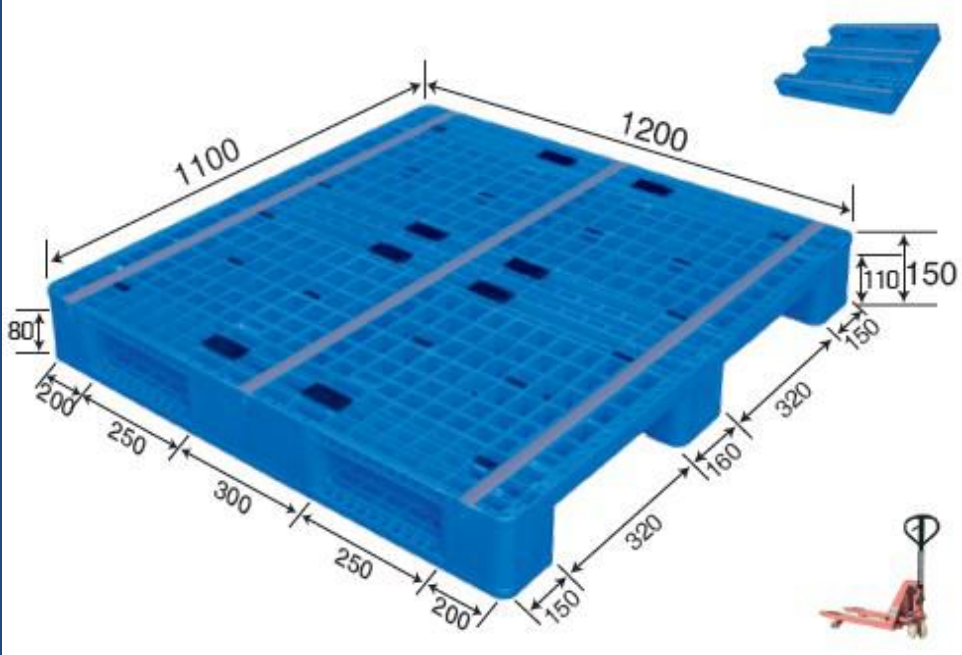
No. 481 MR - 1211D Three Runner (Steel reinforced)
