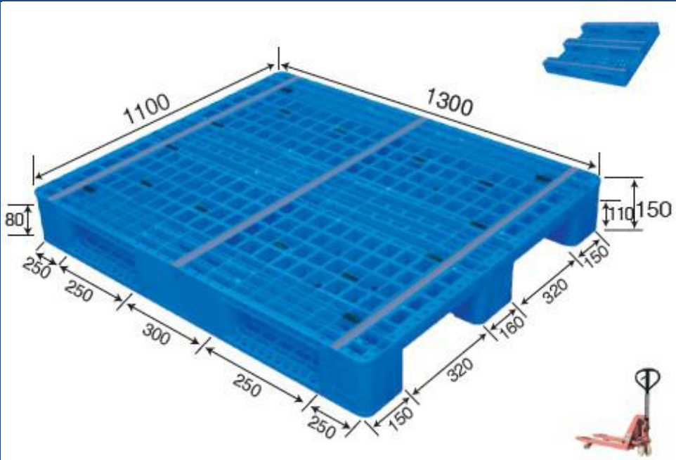
No. 538 MR - 1311D Three Runner (Steel reinforced)
