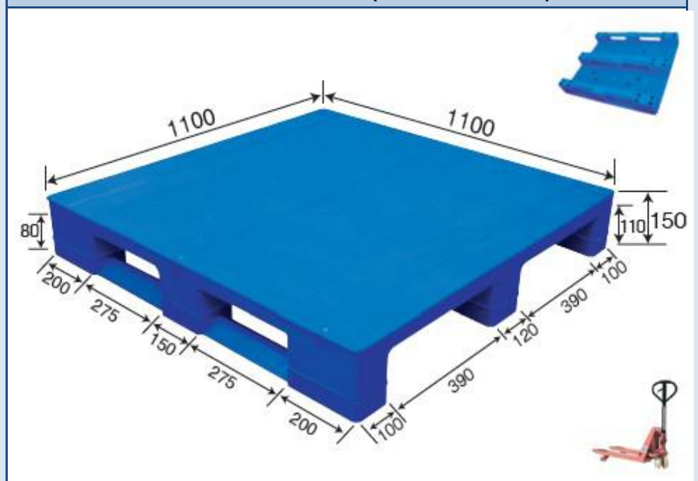
No. 172 MR - 1111 Flat Three Runner (Steel reinforced)
