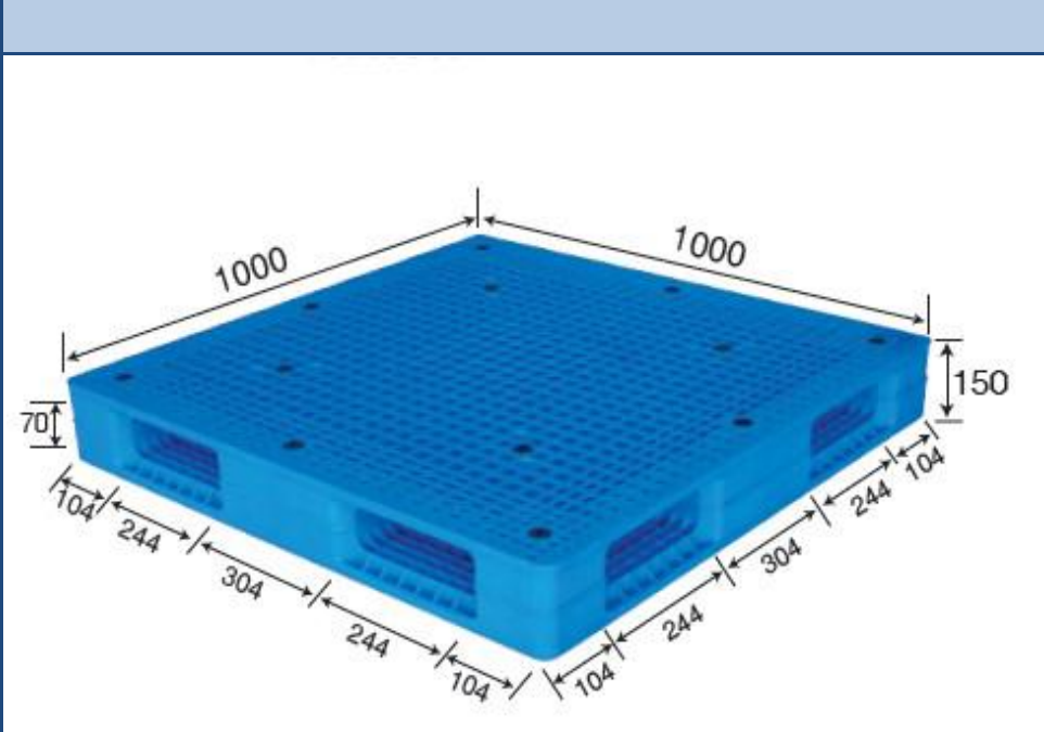
No. 840 MR - 1010 Reversible
