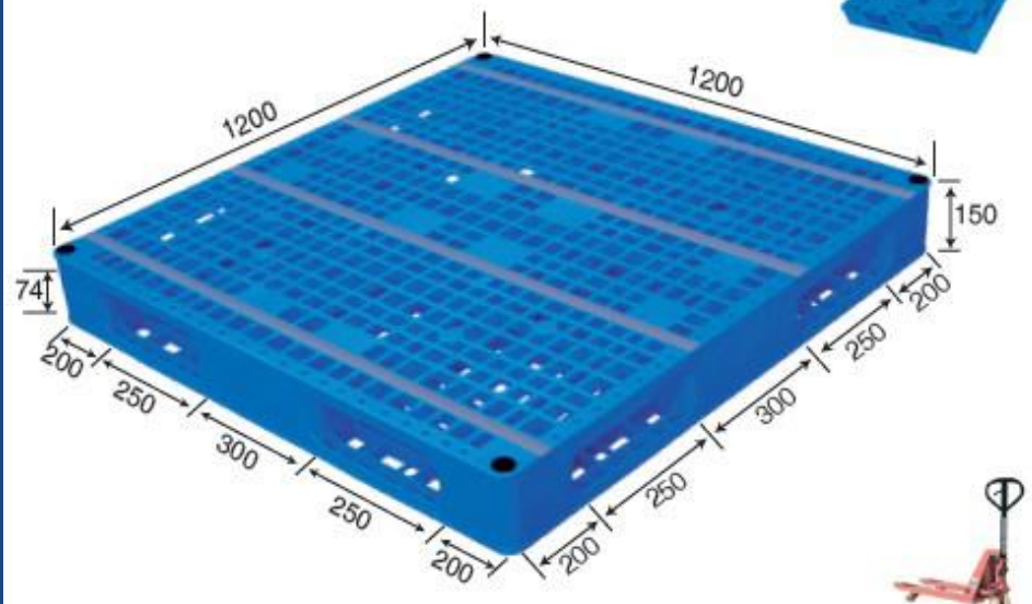
No. 413 MR - 1212D Double Deck (Steel reinforced)
