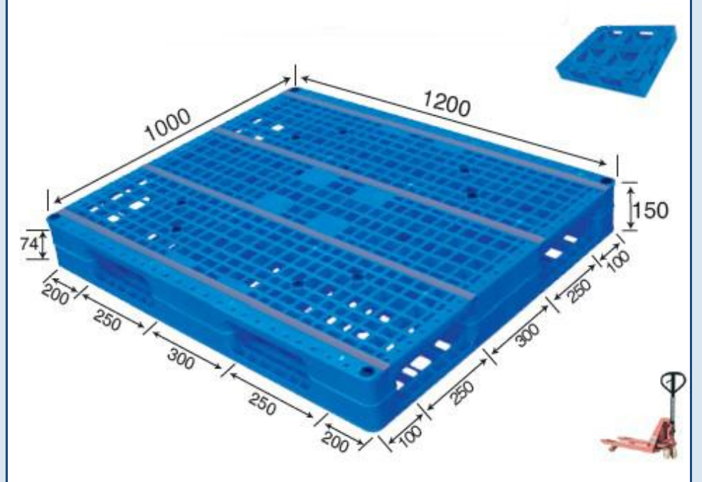
No. 98 MR - 1210D Double Deck (Steel reinforced)
