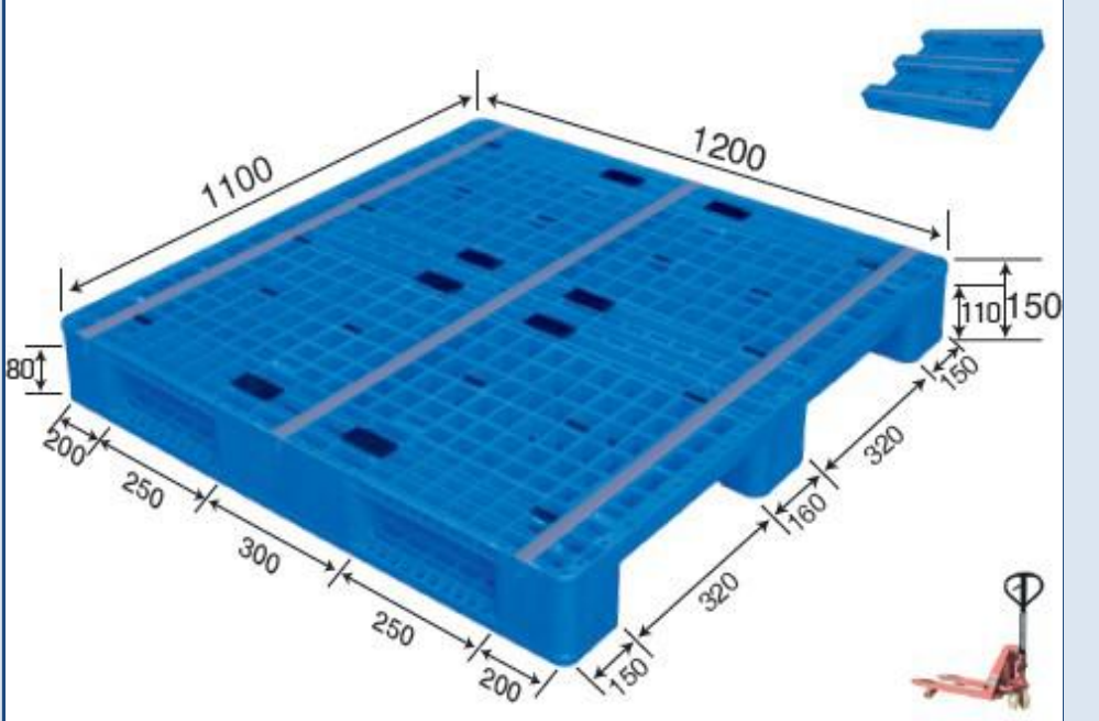
No. 482 MR - 1211D Three Runner (Steel reinforced)
