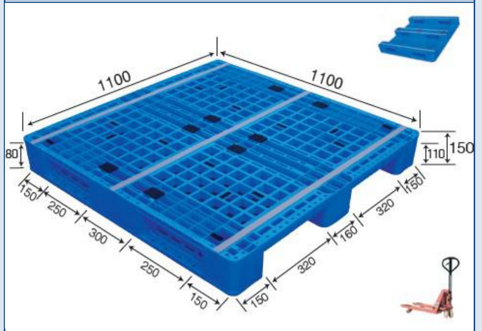
No. 169 MR - 1111D Three Runner (Steel reinforced)
