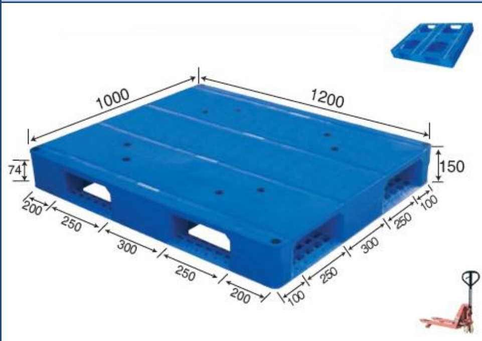
No. 99 MR - 1210D Flat Double Deck (Steel reinforced)
