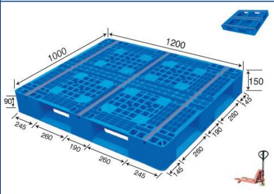
No. 102 MR - 1210D Double Deck (Steel reinforced)
