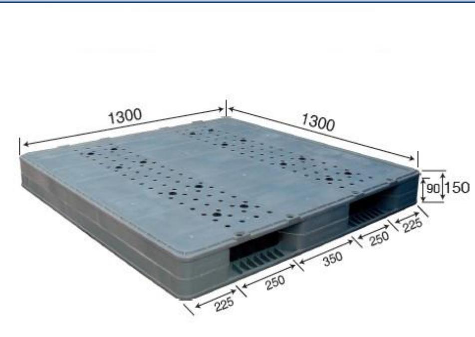
No. 684 MR - 1313 Flat Reversible
