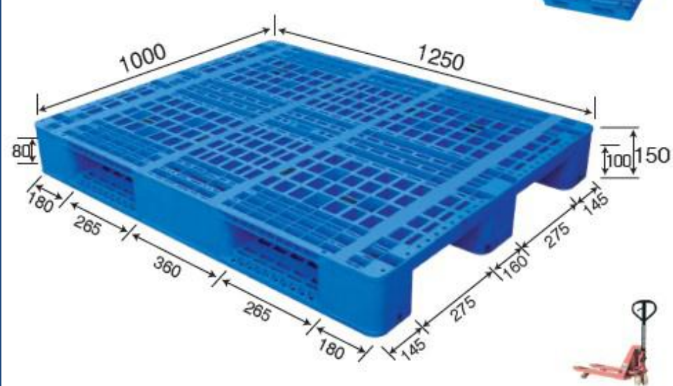
No. 465 MR - 12510D Three Runner (Steel reinforced)
