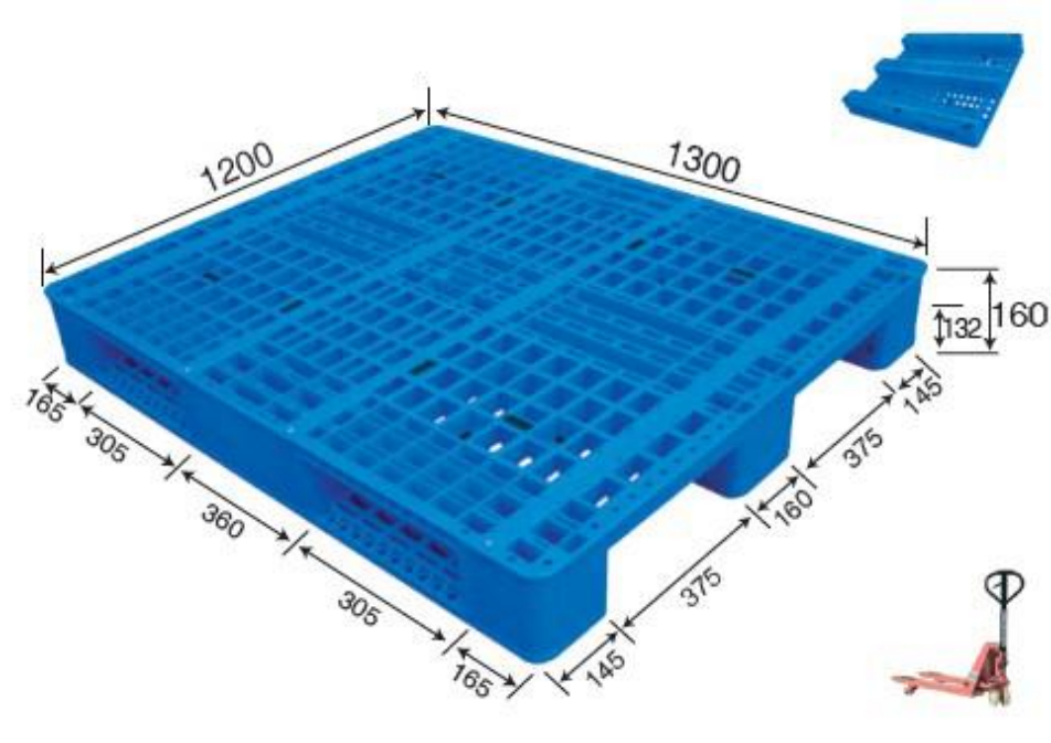
No. 665 MR - 1312D Three Runner (Steel reinforced)
