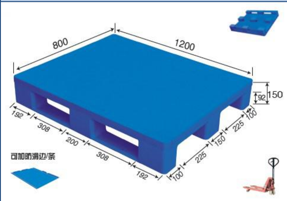
No. 691 MR - 1208 Flat Three Runner (Steel reinforced)
