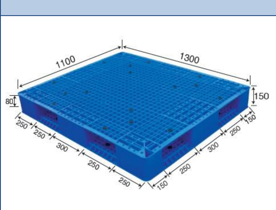
No. 577 MR - 1311 Reversible
