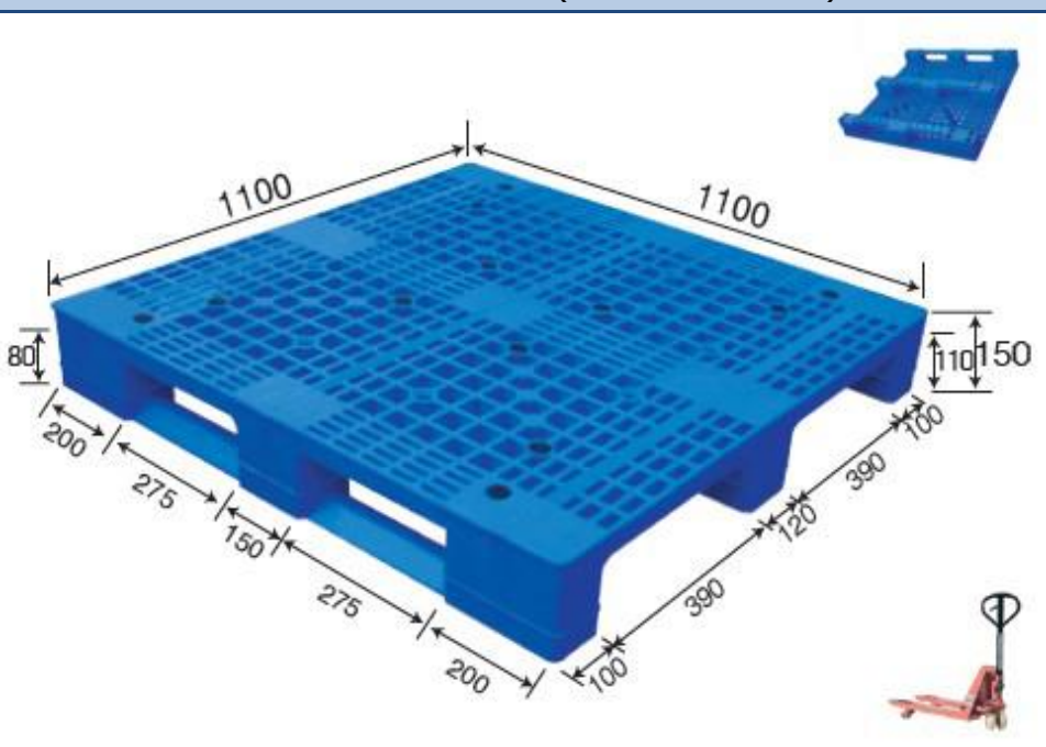
No. 171 MR - 1111 Three Runner (Steel reinforced)
