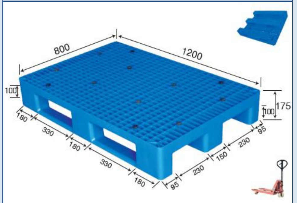
No. 693 MR - 1208TB Three Runner
