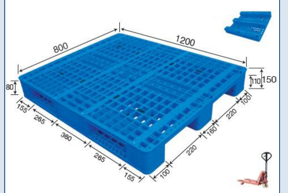
No. 699 MR - 1208D Three Runner
