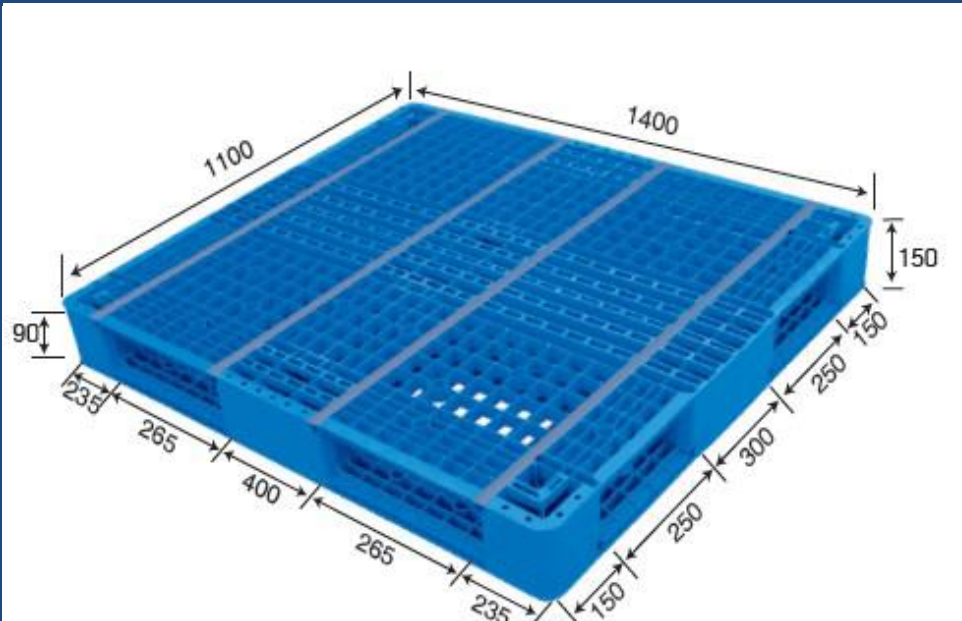
No. 874 MR - 1411D Reversible (Steel reinforced)
