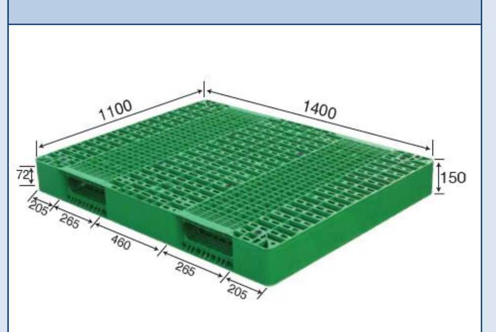
No. 872 MR - 1411 Reversible
