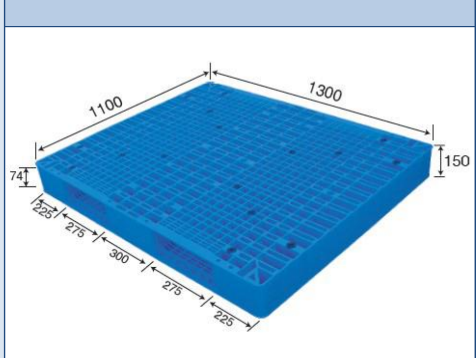
No. 579 MR - 1311 Reversible
