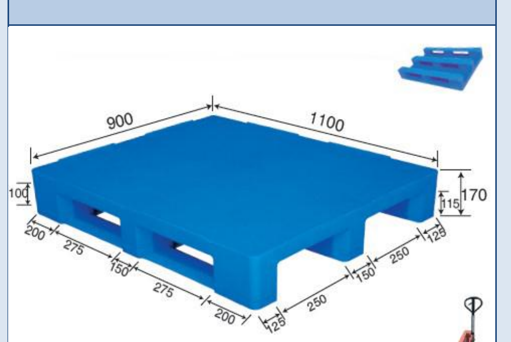
No. 752 MR - 1109 Flat Three Runner
