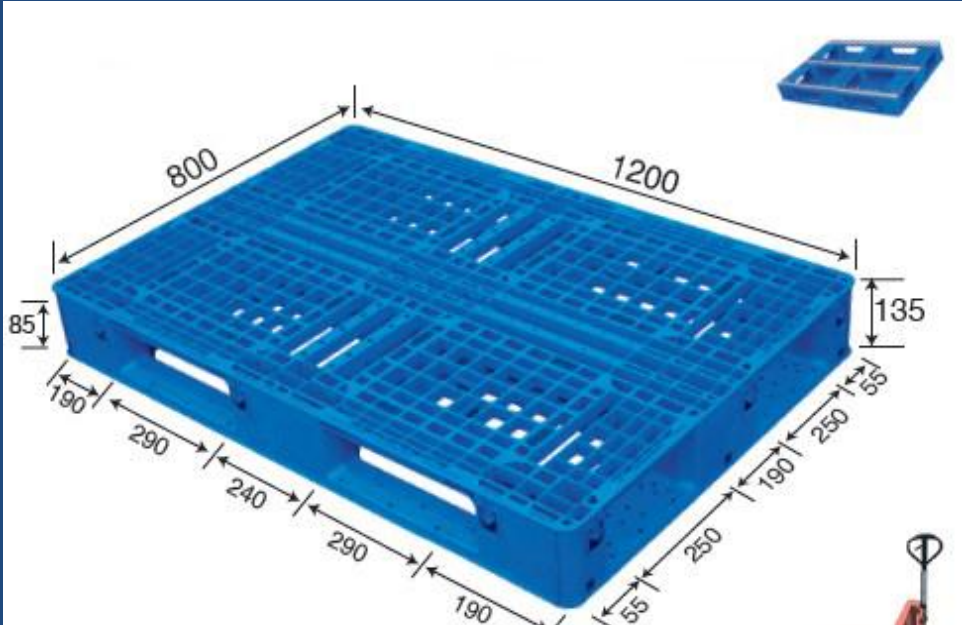
No. 718 MR - 1208 Double Deck (Steel reinforced)
