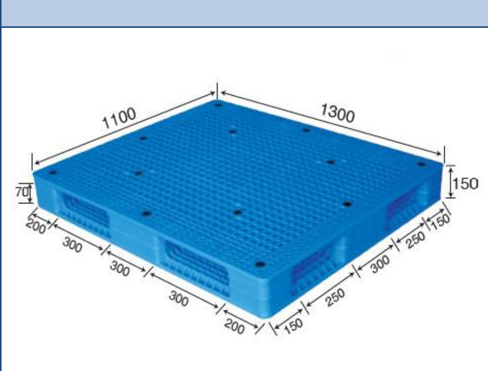
No. 580 MR - 1311 Reversible
