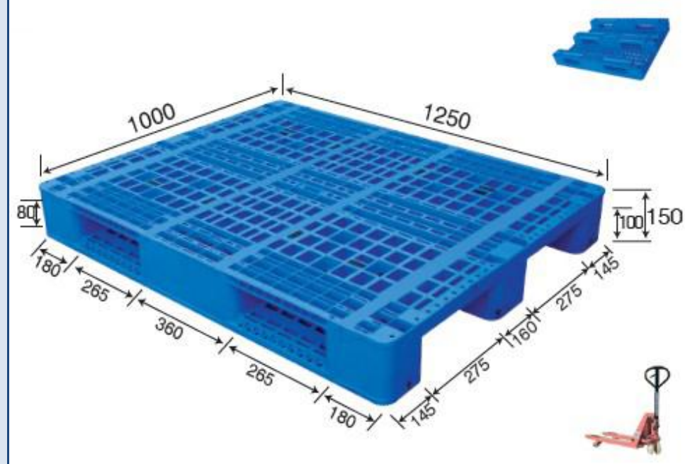
No. 466 MR - 12510D Three Runner (Steel reinforced)
