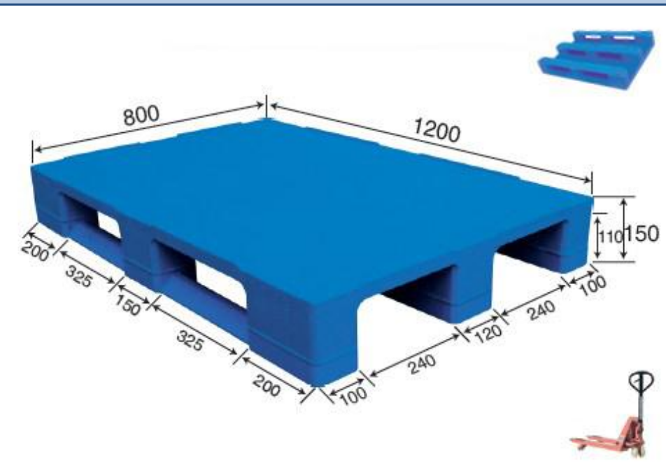
No. 695 MR - 1208 Flat Three Runner (Steel reinforced)
