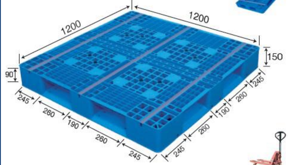
No. 410 MR - 1212D Double Deck (Steel reinforced)
