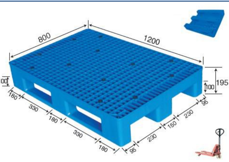
No. 692 MR - 1208T Three Runner
