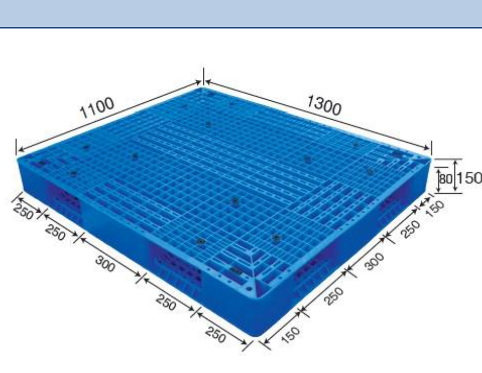
No. 578 MR - 1311B Reversible
