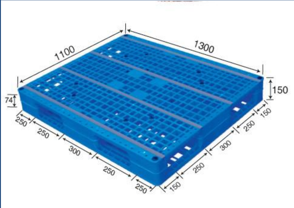
No. 574 MR - 1311D Reversible (Steel reinforced)
