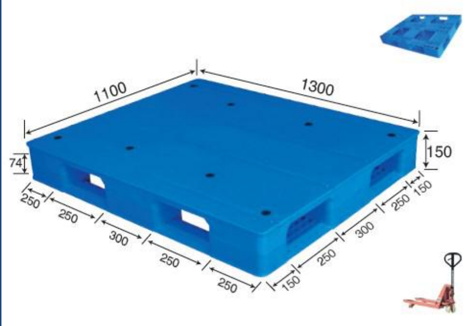
No. 614 MR - 1311D Flat Double Deck (Steel reinforced)
