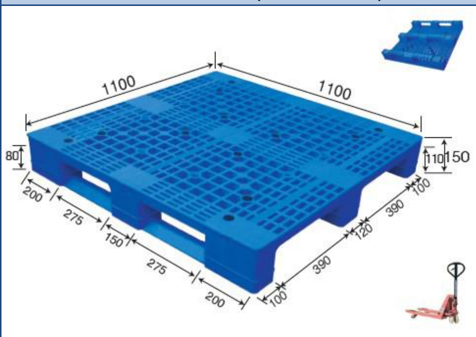
No. 170 MR - 1111 Three Runner (Steel reinforced)
