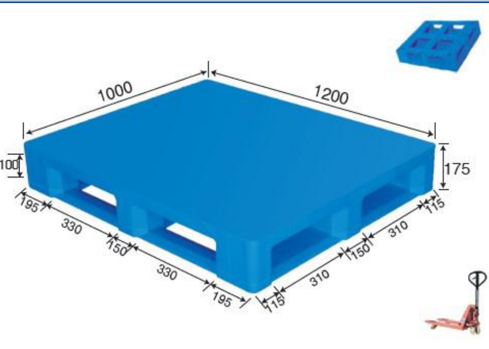
No. 100 MR - 1210 Flat Double Deck
