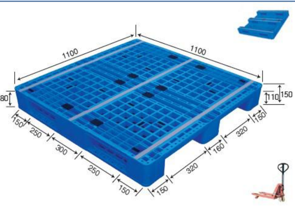
No. 168 MR - 1111D Three Runner (Steel reinforced)
