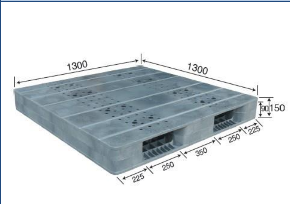
No. 683 MR - 1313 Flat Reversible
