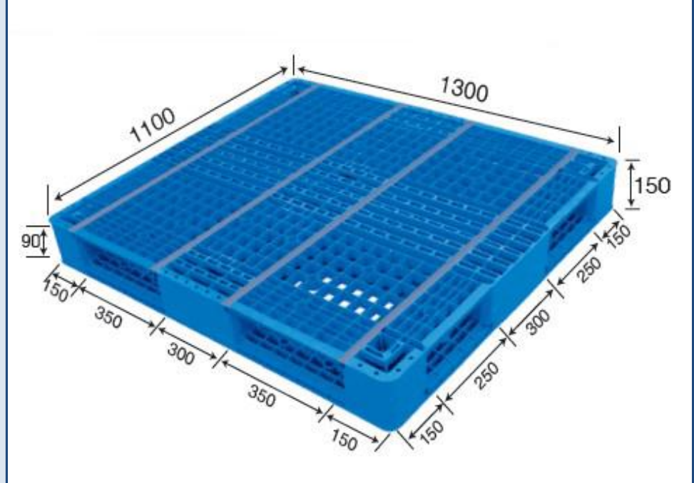
No. 573 MR - 1311D Reversible (Steel reinforced)
