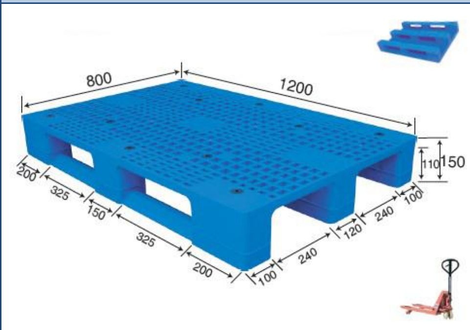
No. 694 MR - 1208 Three Runner (Steel reinforced)
