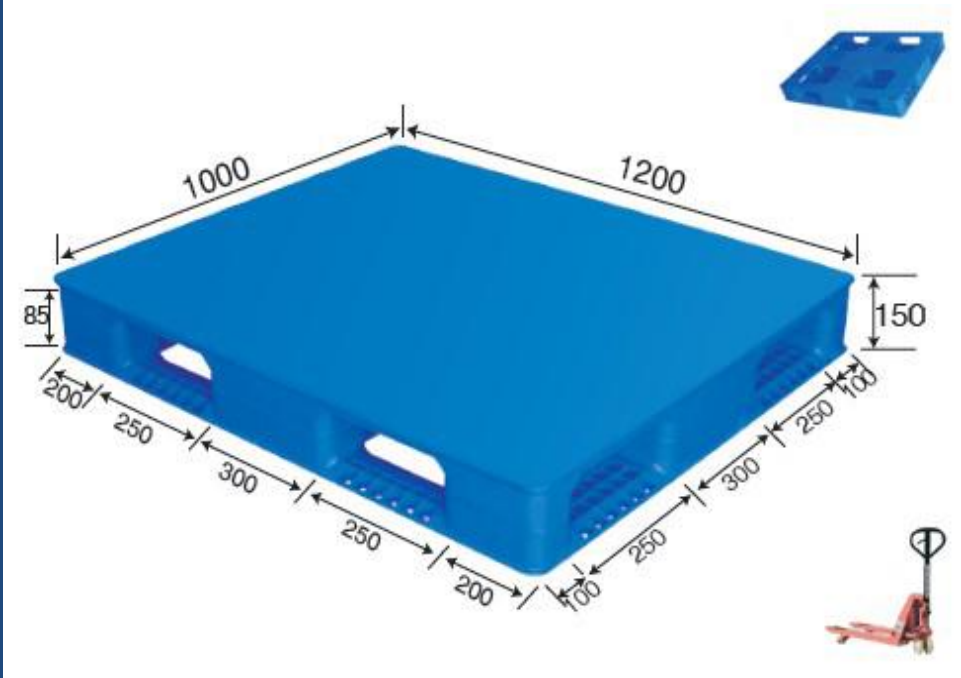
No. 96 MR - 1210 Flat Double Deck (Steel reinforced)
