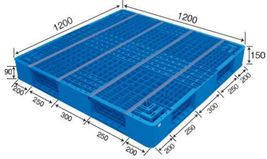
No. 377 MR - 1212D Reversible (Steel reinforced)
