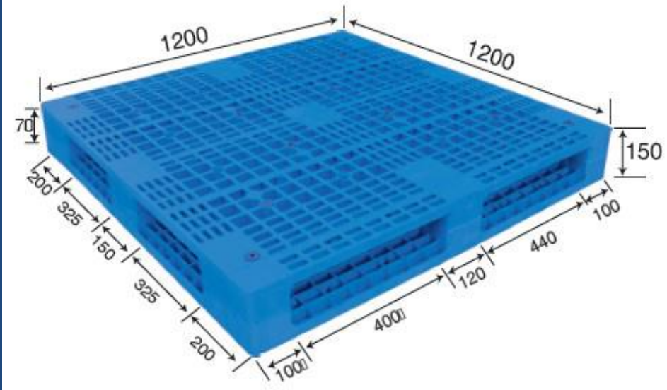
No. 373 MR - 1212 Reversible (Steel reinforced)
