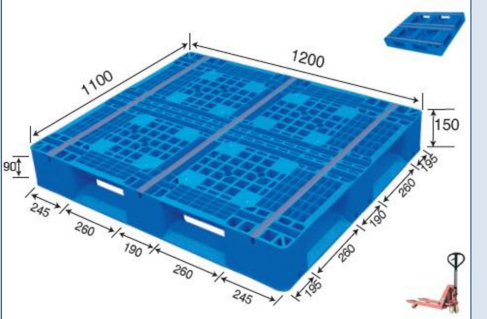
No. 517 MR - 1211D Double Deck (Steel reinforced)
