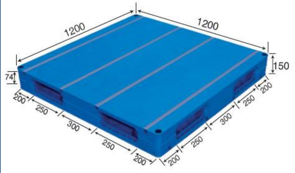
No. 376 MR - 1212D Flat Reversible (Steel reinforced)
