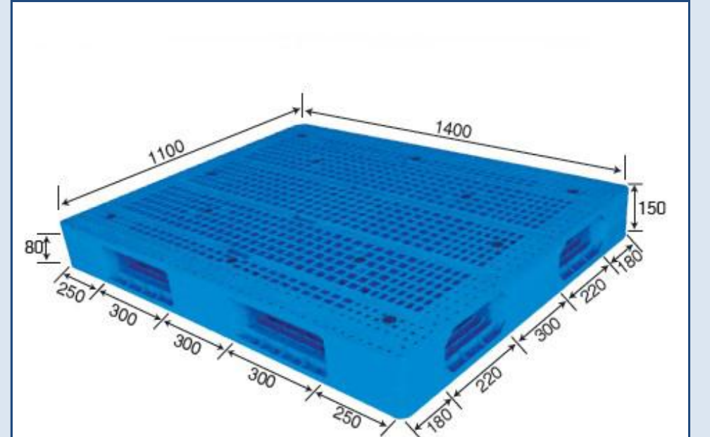
No. 875 MR - 1411D Reversible (Steel reinforced) (Welded)
