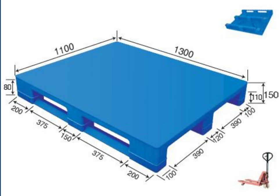
No. 543 MR - 1311 Flat Three Runner (Steel reinforced)
