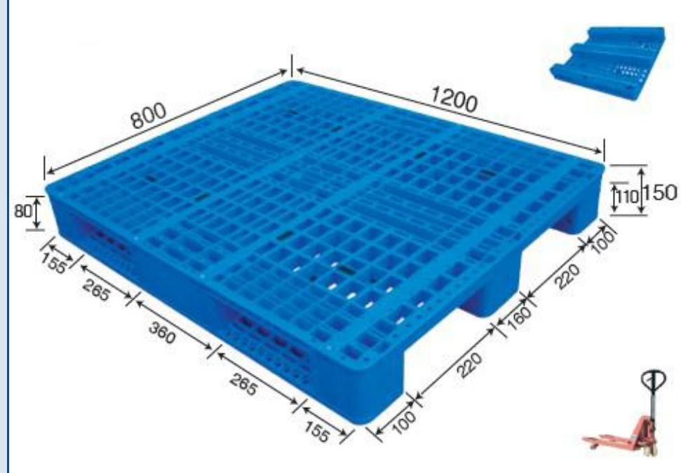
No. 697 MR - 1208D Three Runner (Steel reinforced)
