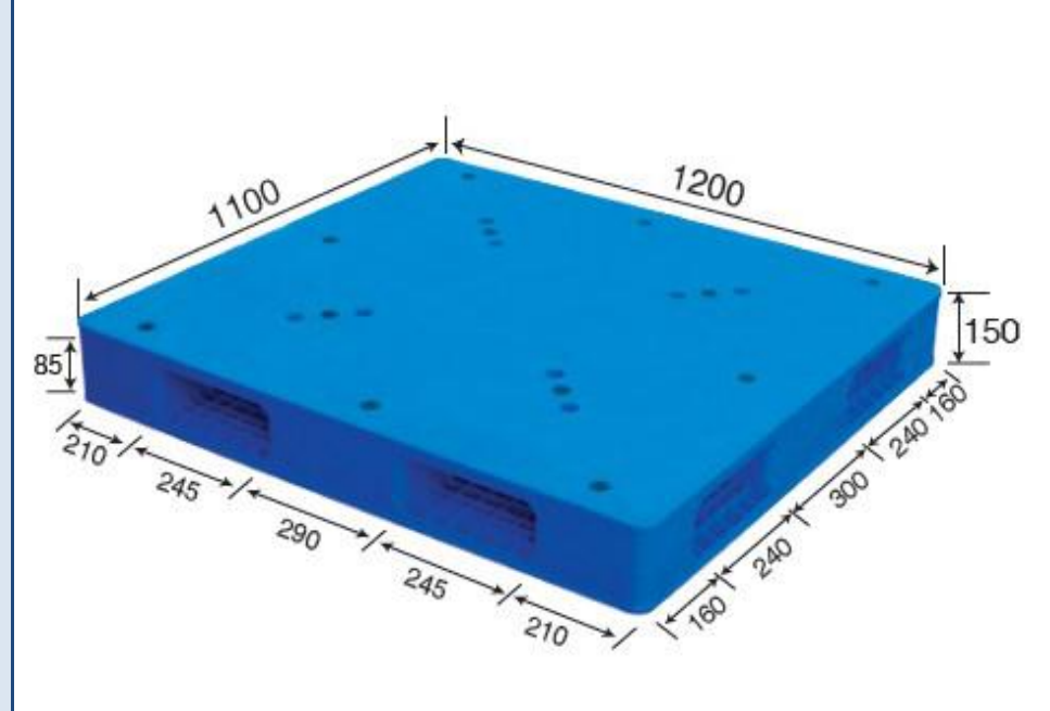
No. 500 MR - 1211 Flat Reversible (Steel reinforced)
