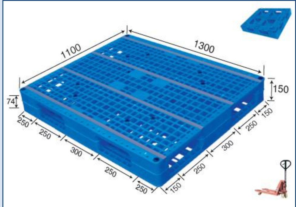
No. 613 MR - 1311D Double Deck (Steel reinforced)
