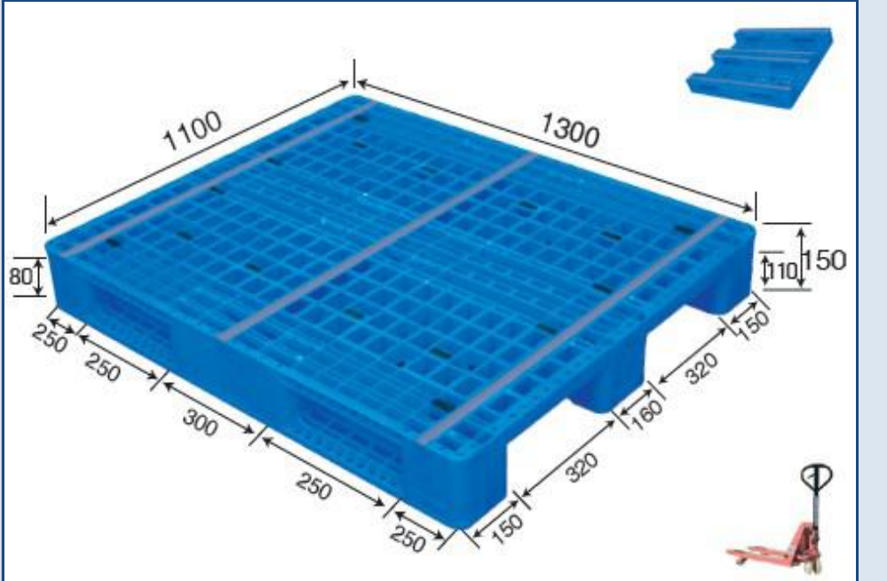
No. 539 MR - 1311D Three Runner (Steel reinforced)
