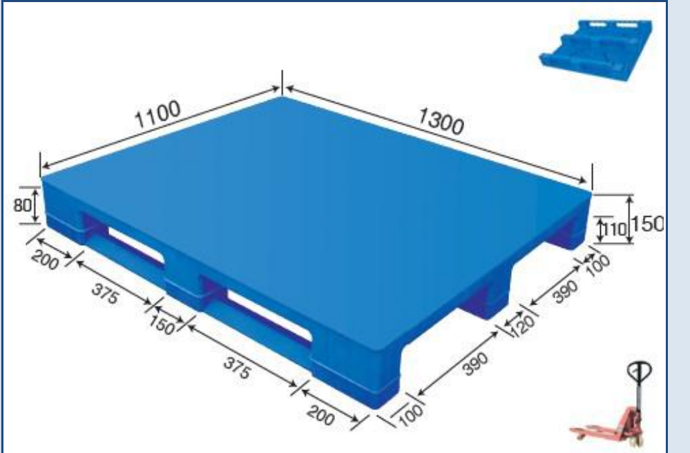
No. 542 MR - 1311 Flat Three Runner (Steel reinforced)
