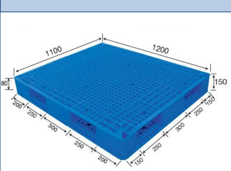
No. 501 MR - 1211 Reversible
