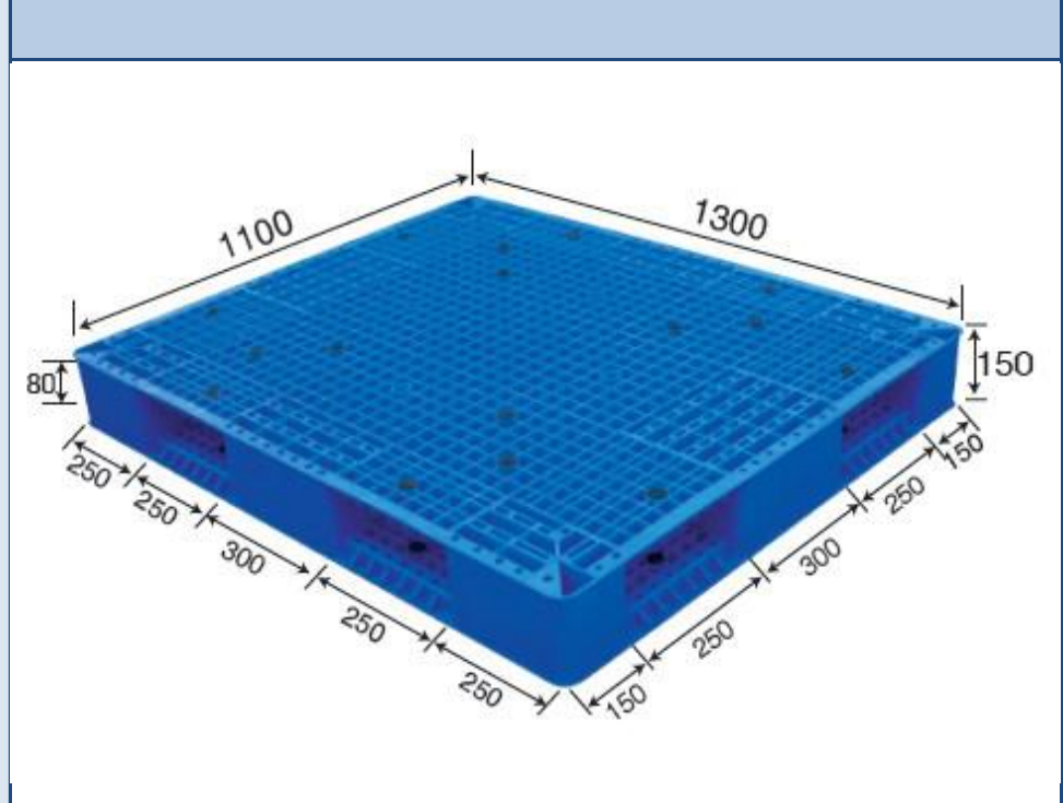
No. 576 MR - 1311 Reversible
