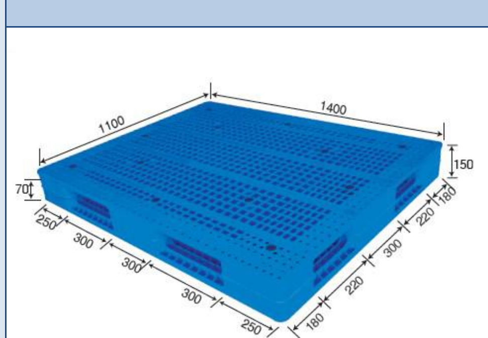
No. 873 MR - 1411 Reversible
