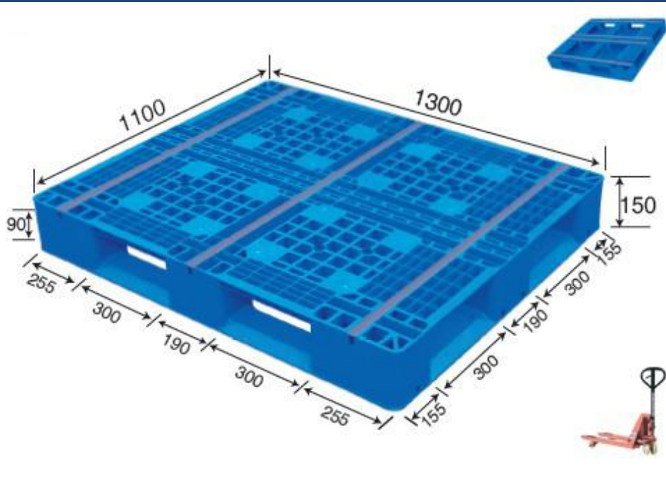
No. 612 MR - 1311D Double Deck (Steel reinforced)
