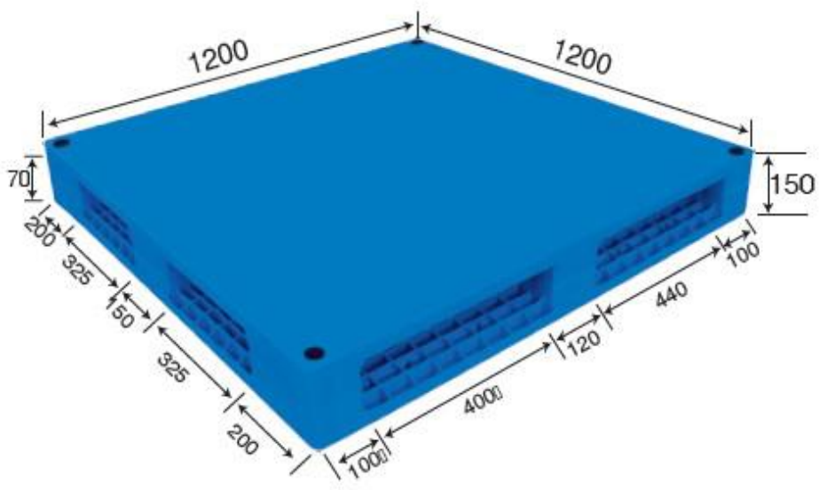
No. 374 MR - 1212 Flat Reversible (Steel reinforced)
