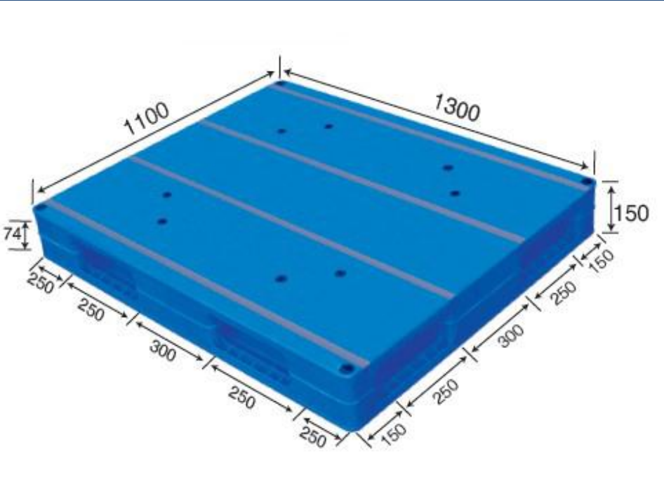
No. 575 MR - 1311D Flat Reversible (Steel reinforced)
