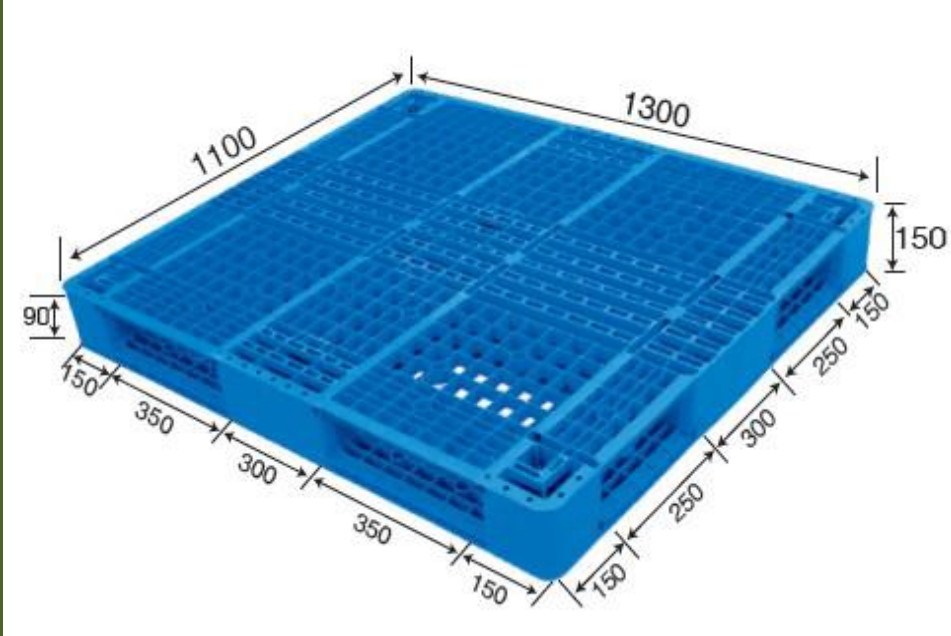
No. 596 MS - 1311D Reversible
