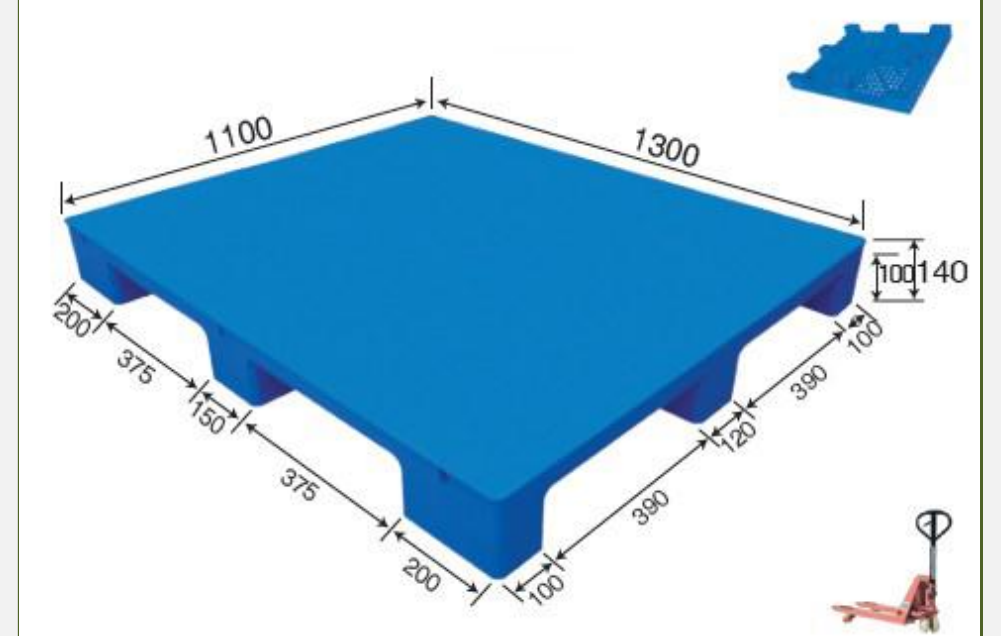
No. 648 MS - 1311A Flat Nine Footer
