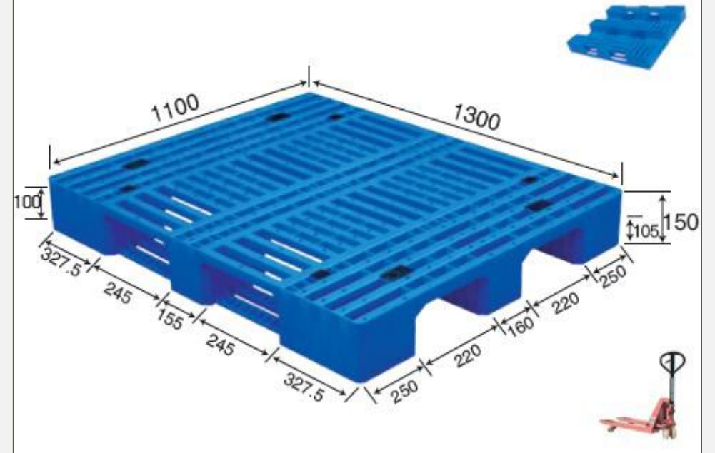
No. 561 MS - 1311A Flat Welding Double Deck (Welded)
