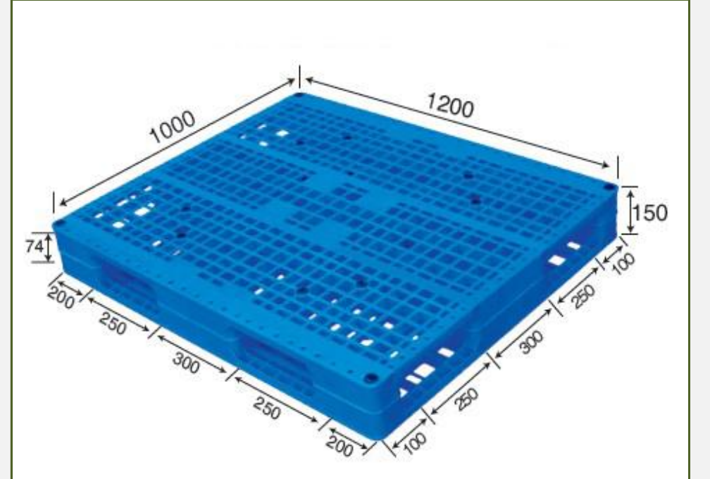
No. 79 MS - 1210D Reversible
