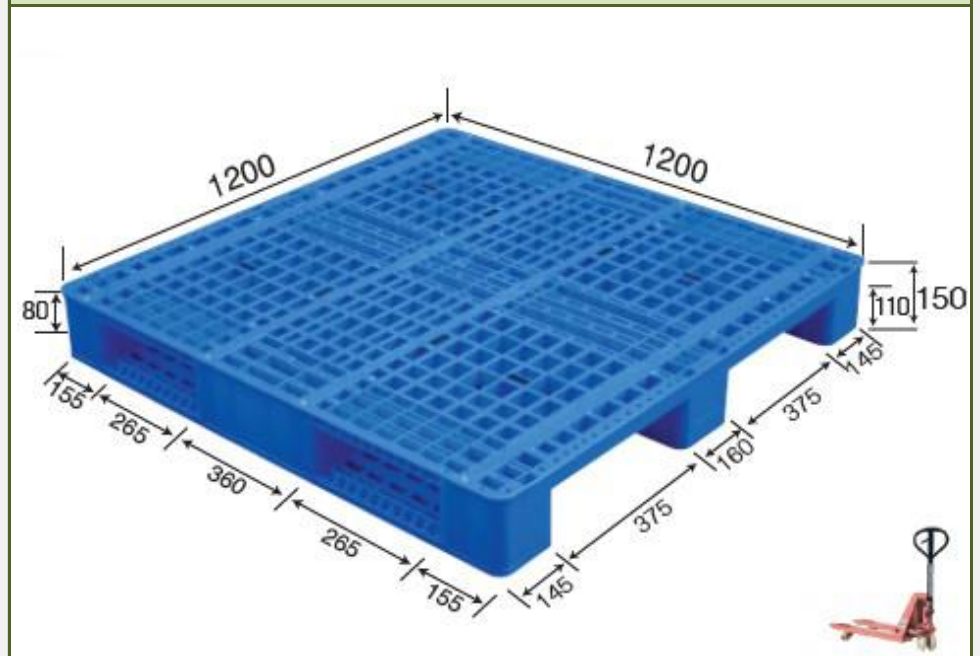
No. 359 MS - 1212D Three Runner
