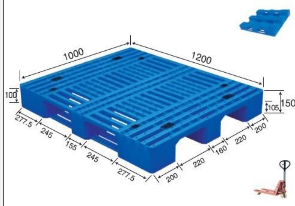
No. 32 MS - 1210A Three Runner
