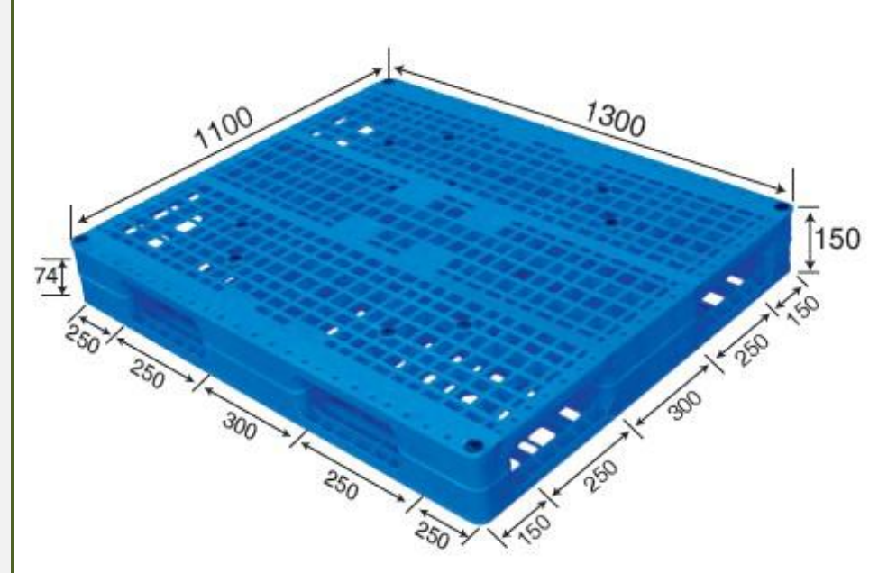
No. 597 MS - 1311D Reversible
