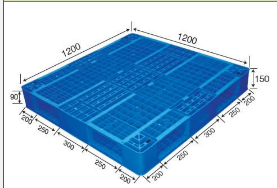
No. 393 MS - 1212D Reversible
