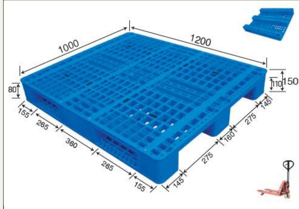
No. 35 MS - 1210D Three Runner
