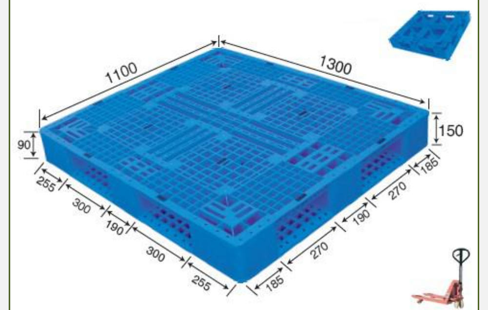
No. 631 MS - 1311 Double Deck
