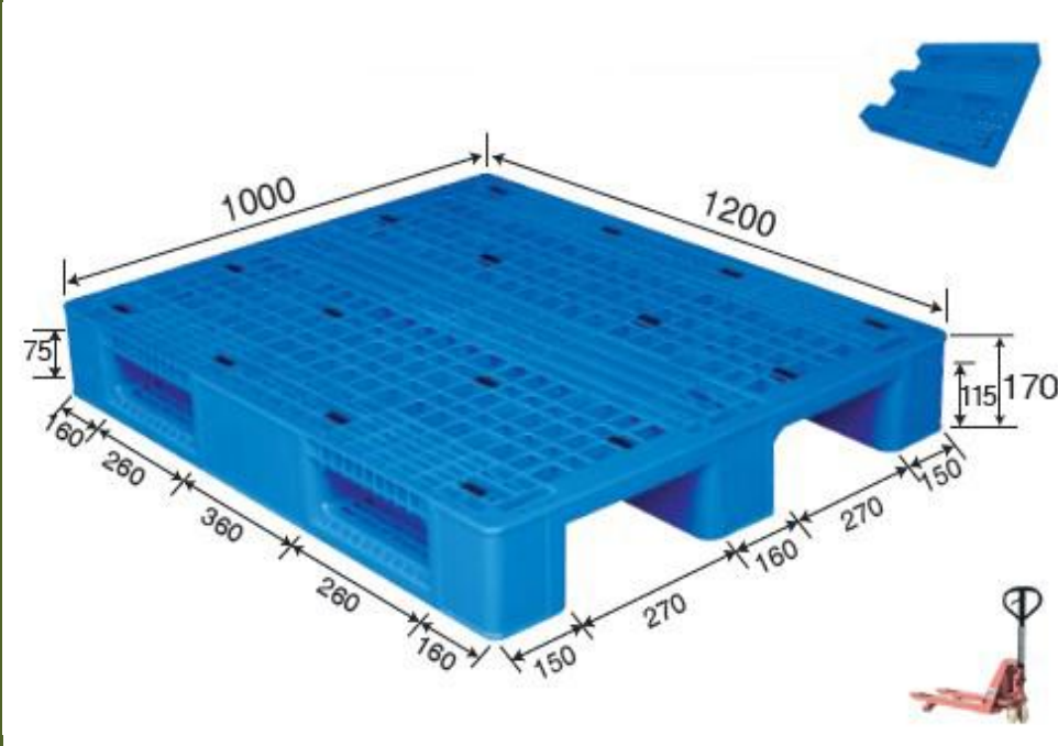
No. 33 MS - 1210B Three Runner
