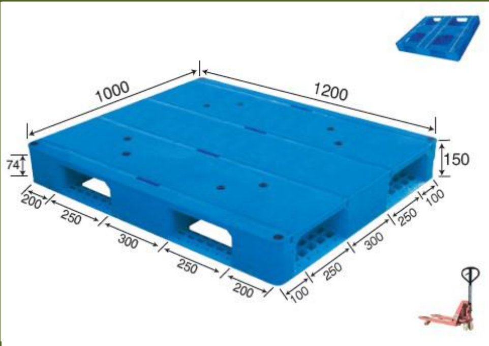
No. 124 MS - 1210D Flat Double Deck (Welded)
