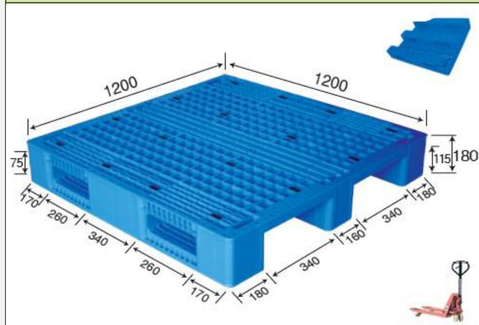
No. 357 MS - 1212B Three Runner
