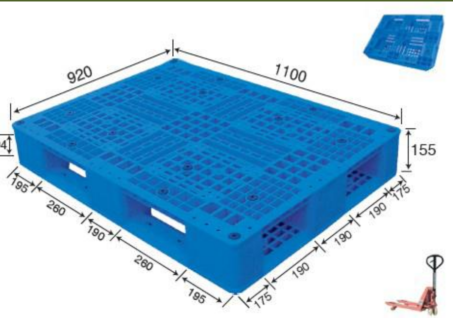
No. 790 MS - 1109 Double Deck
