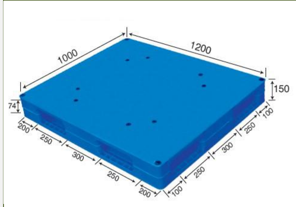
No. 80 MS - 1210D Flat reversible
