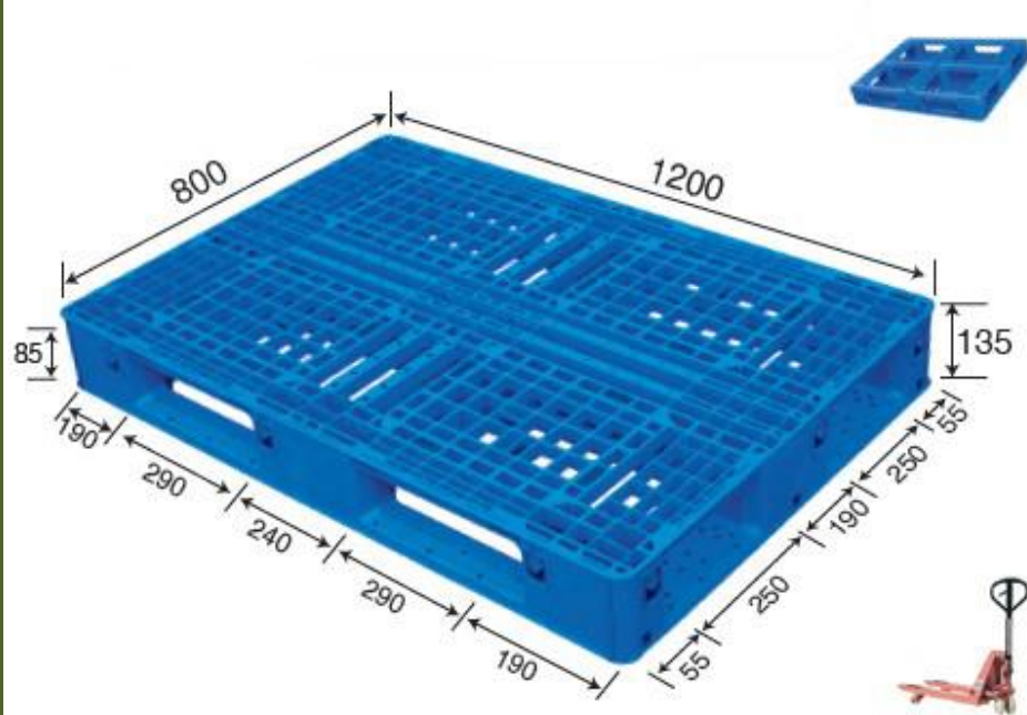
No. 729 MS - 1208 Double Deck
