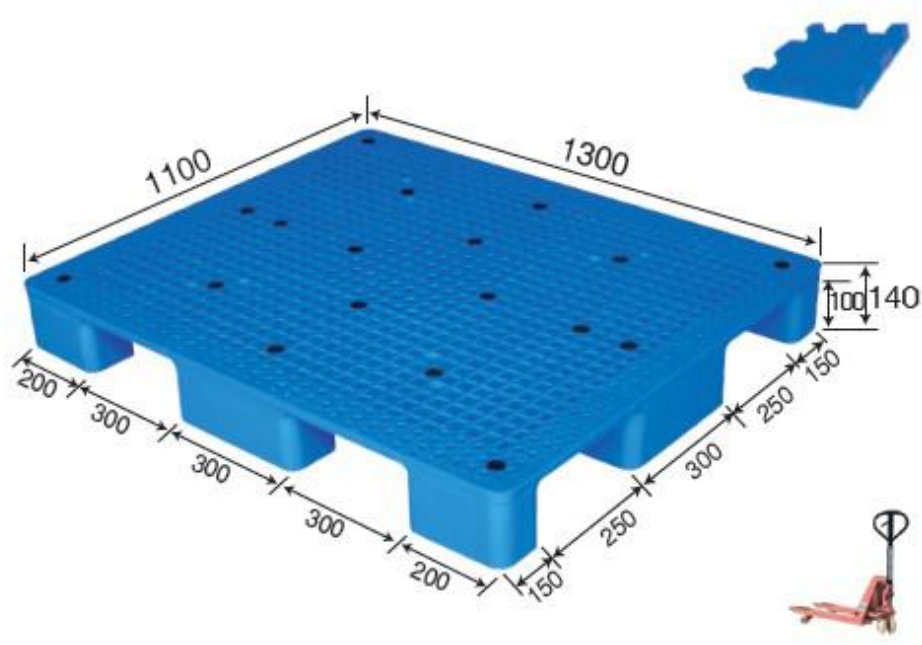
No. 649 MS - 1311 Nine Footer
