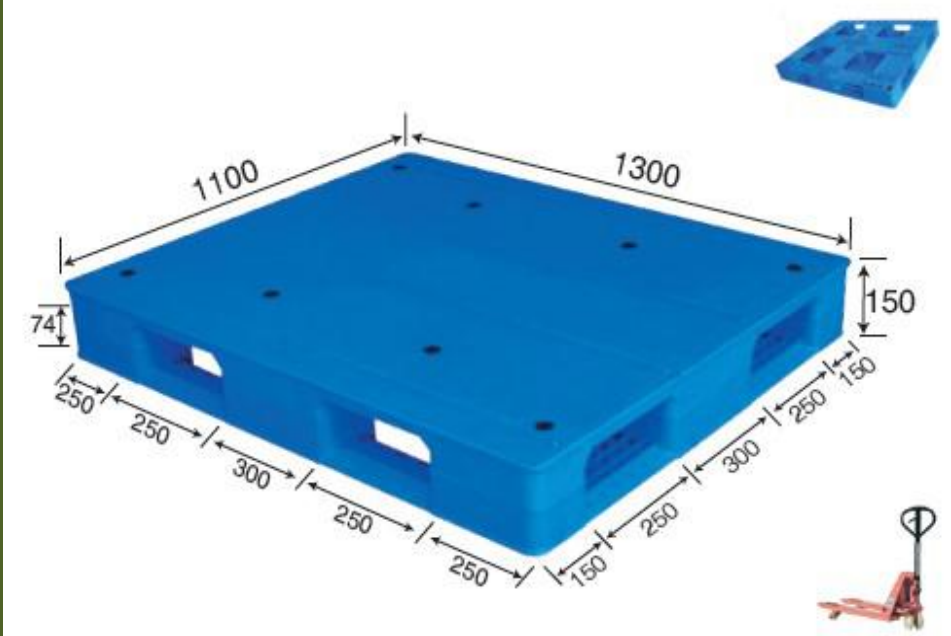
No. 632 S - 1311D Flat Double Deck (Welded)
