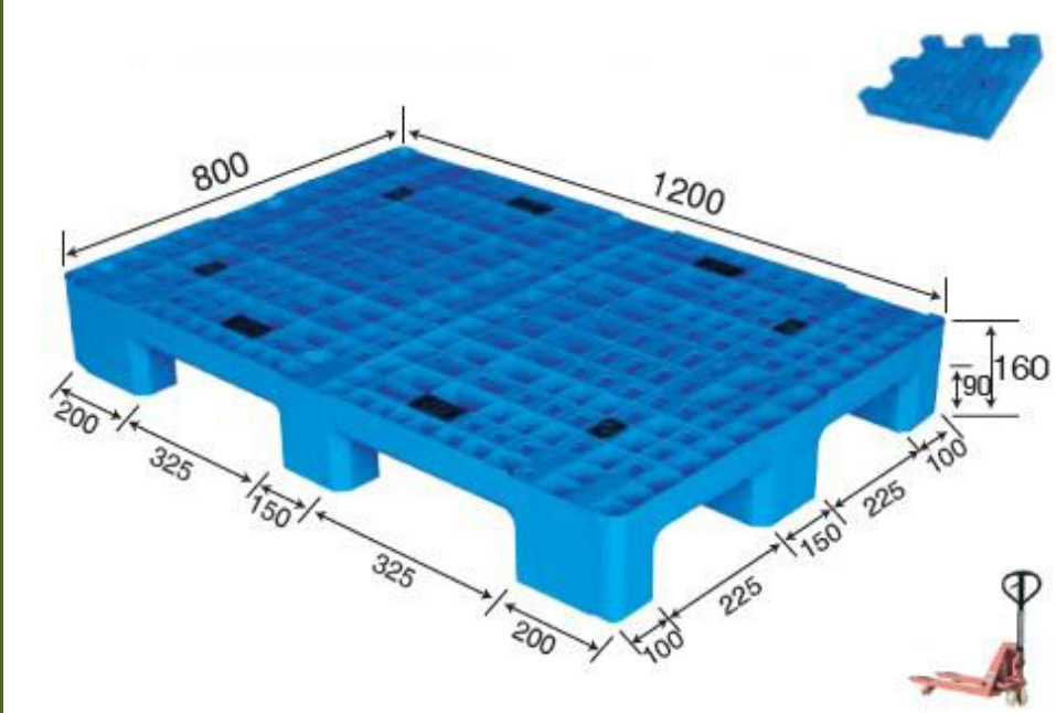
No. 738 MS - 1208 Nine Footer
