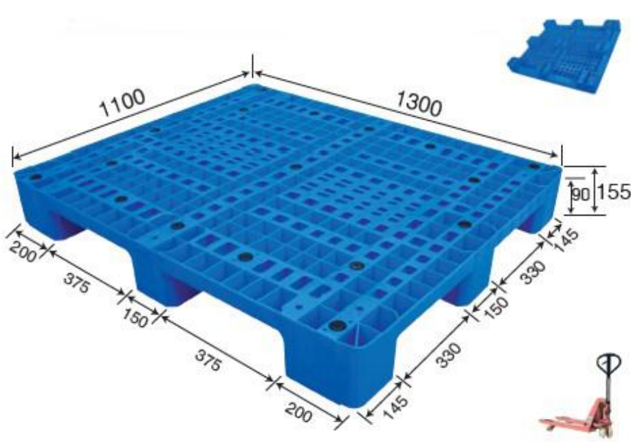
No. 650 MS - 1311B Nine Footer
