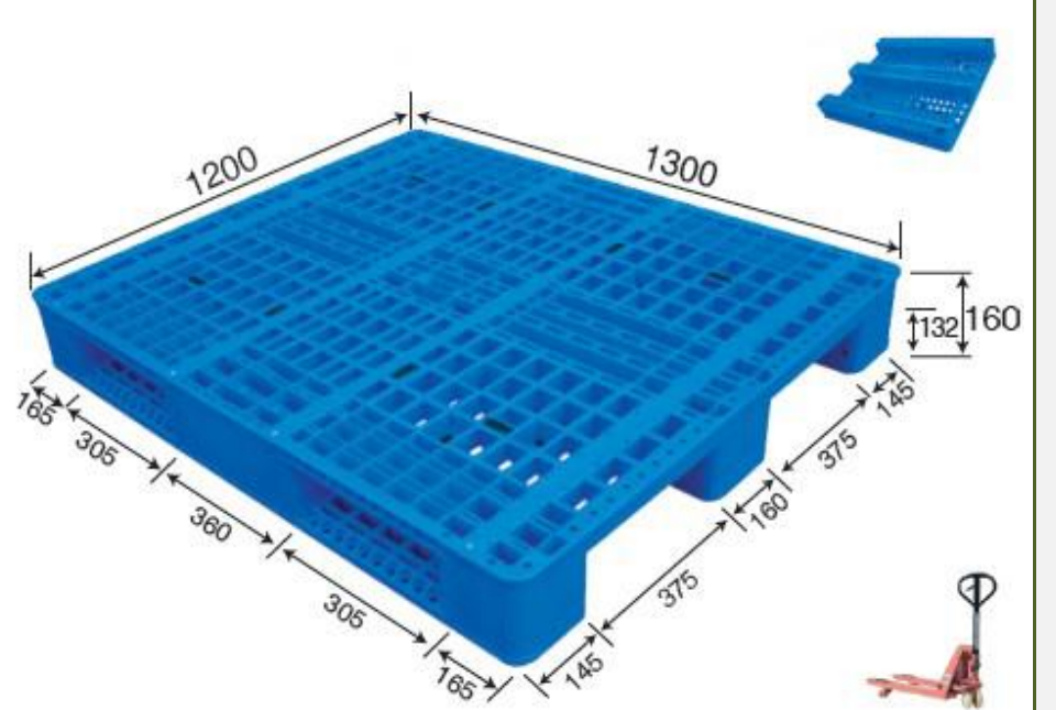
No. 671 MS - 1312D Three Runner
