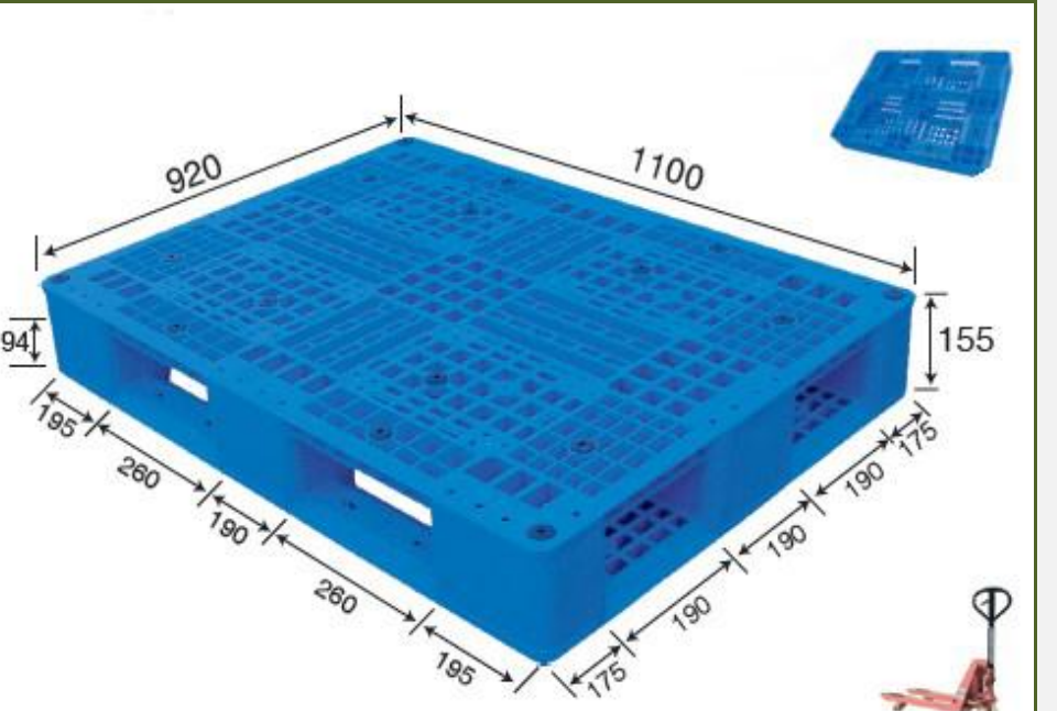
No. 791 MS - 1109 Double Deck
