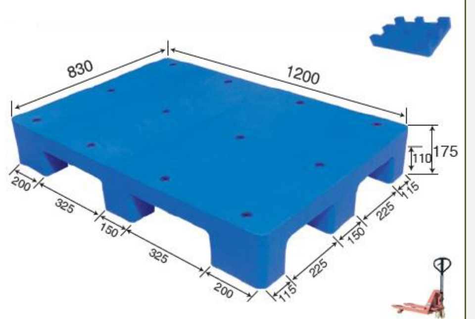
No. 740 MS - 12083 Flat Nine Footer
