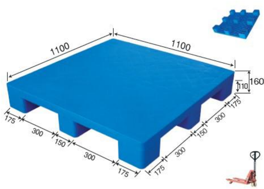
No. 294 MS - 1111A Flat Nine Footer
