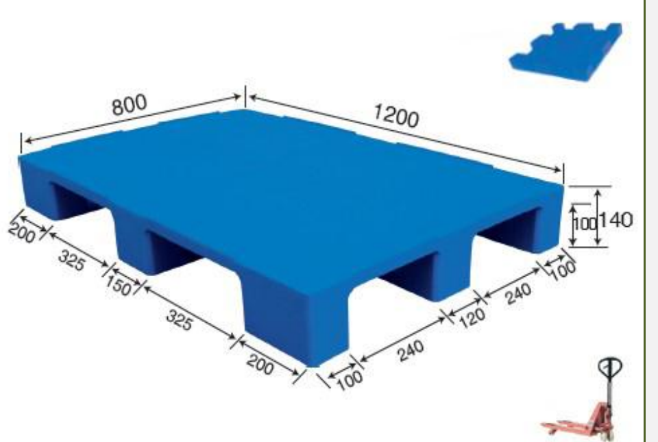
No. 737 MS - 1208A Flat Nine Footer
