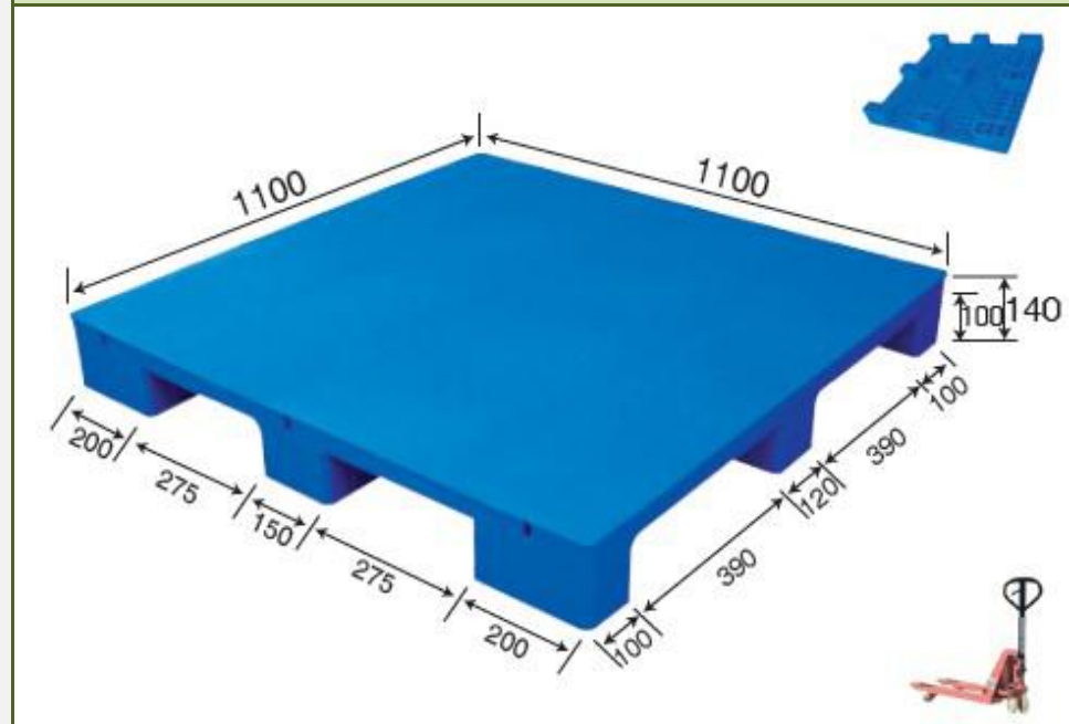
No. 296 MS - 1111C Flat Nine Footer
