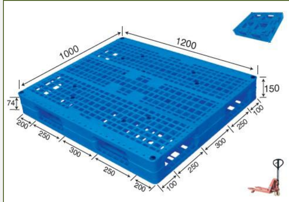
No. 123 MS - 1210D Double Deck (Welded)
