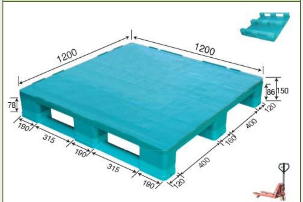
No. 356 MS - 1212 Flat Three Runner
