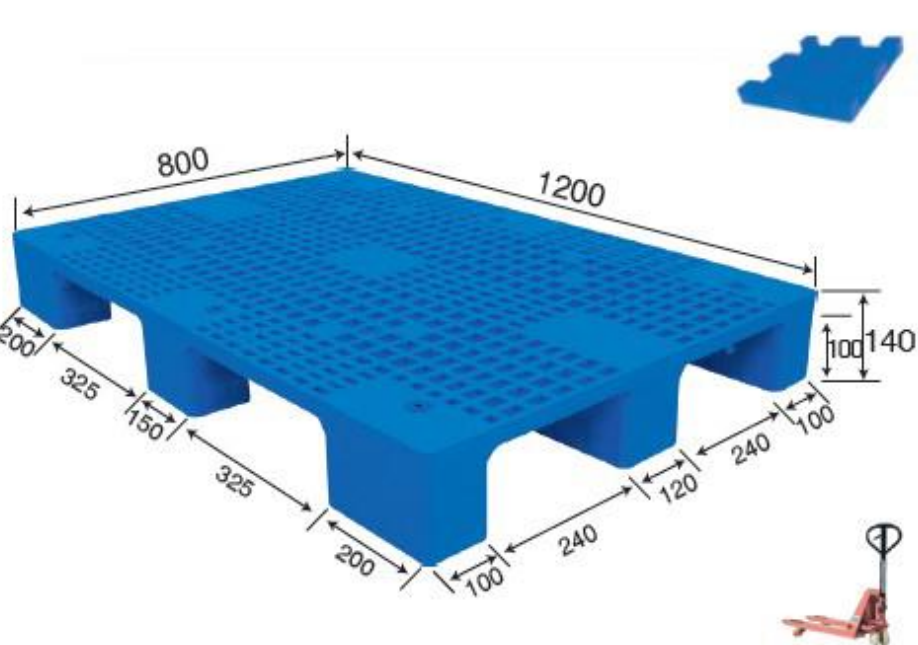
No. 736 MS - 1208A Nine Footer
