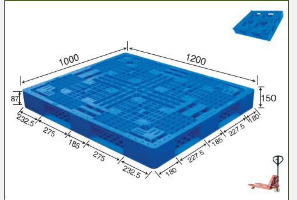
No. 125 MS - 1210 Double Deck
