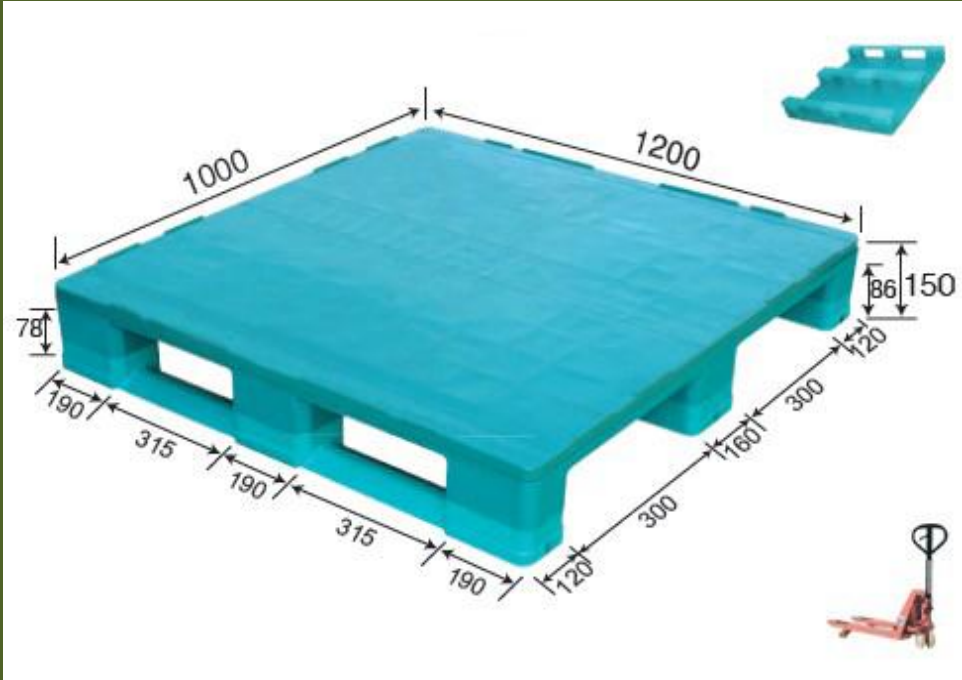
No. 36 MS - 1210 Flat Three Runner
