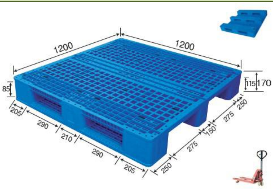
No. 358 MS - 1212C Three Runner
