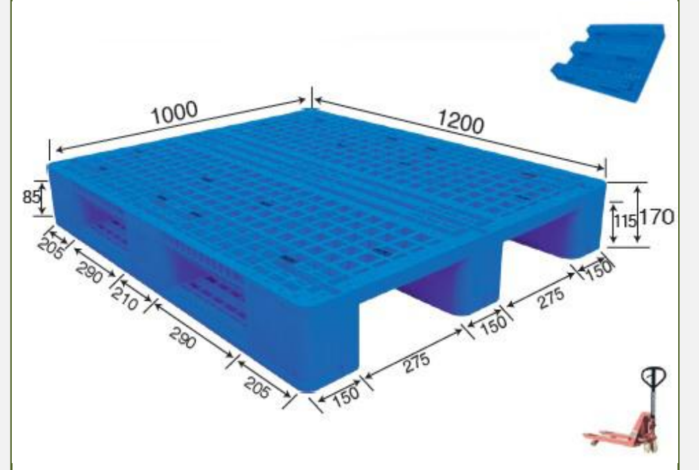
No. 34 MS - 1210C Three Runner
