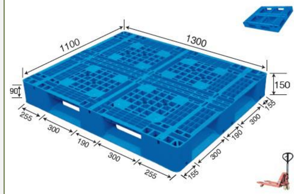
No. 630 MS - 1311D Double Deck
