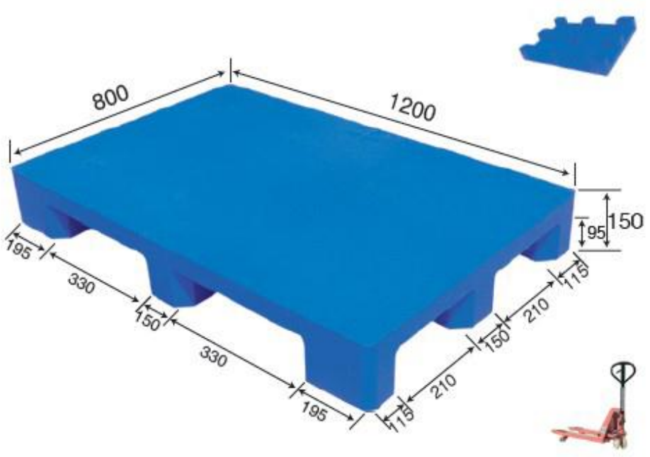
No. 739 MS - 1208 Flat Nine Footer
