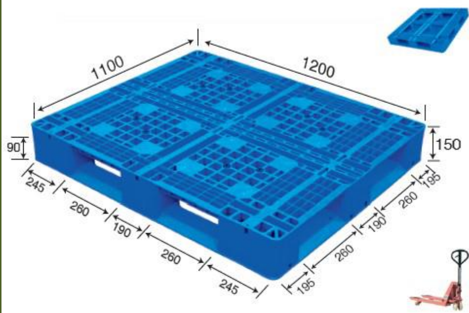
No. 528 MS - 1211D Double Deck
