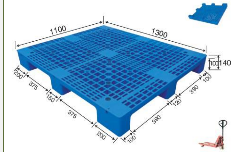
No. 647 S - 1311A Nine Footer
