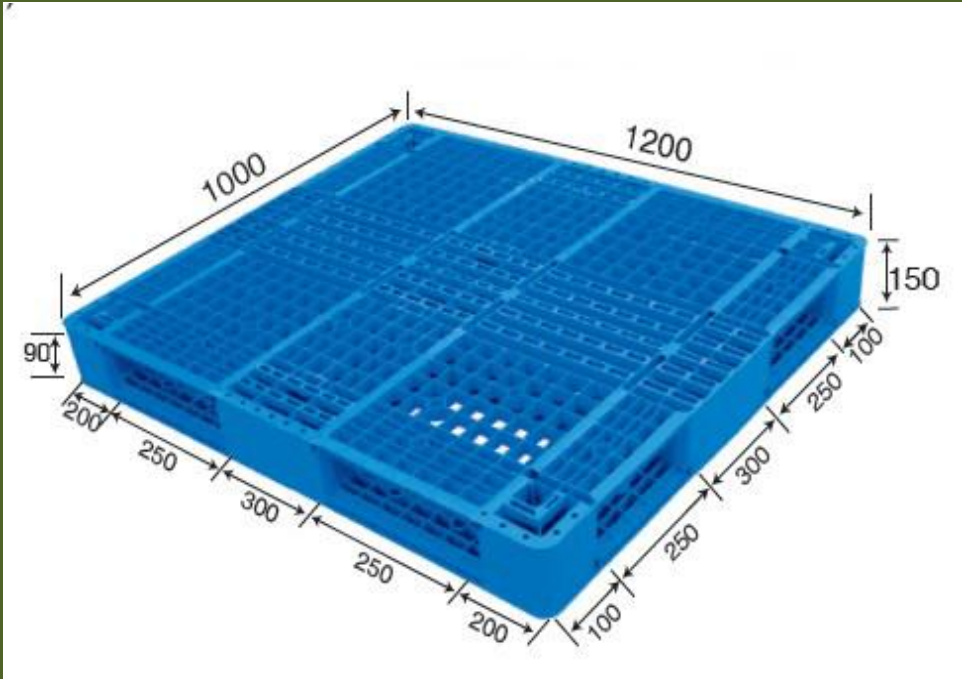
No. 81 MS - 1210D Reversible
