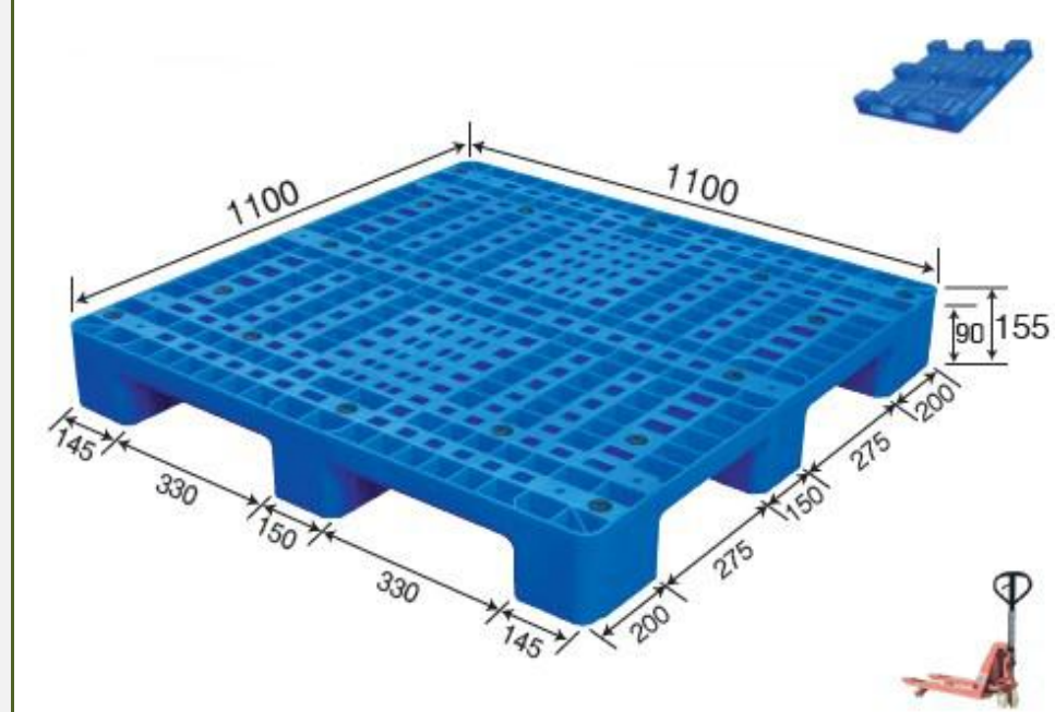
No. 293 MS - 1111B Nine Footer
