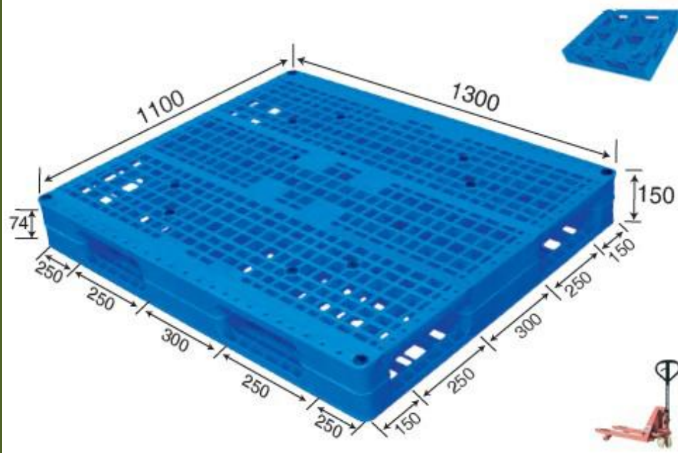
No. 629 MS - 1311D Double Deck (Welded)
