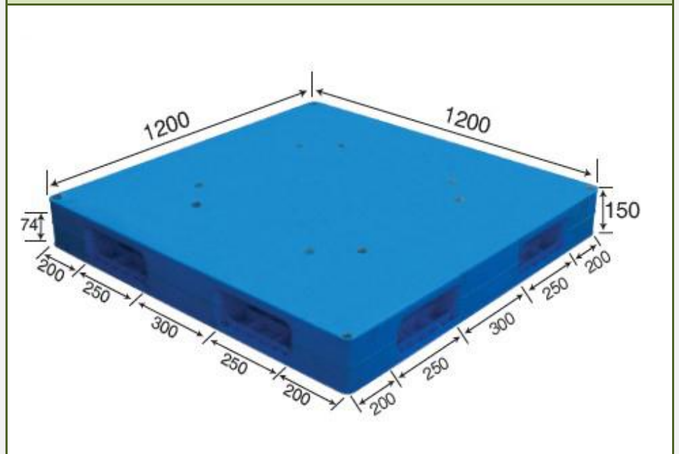
No. 395 MS - 1212D Flat Reversible
