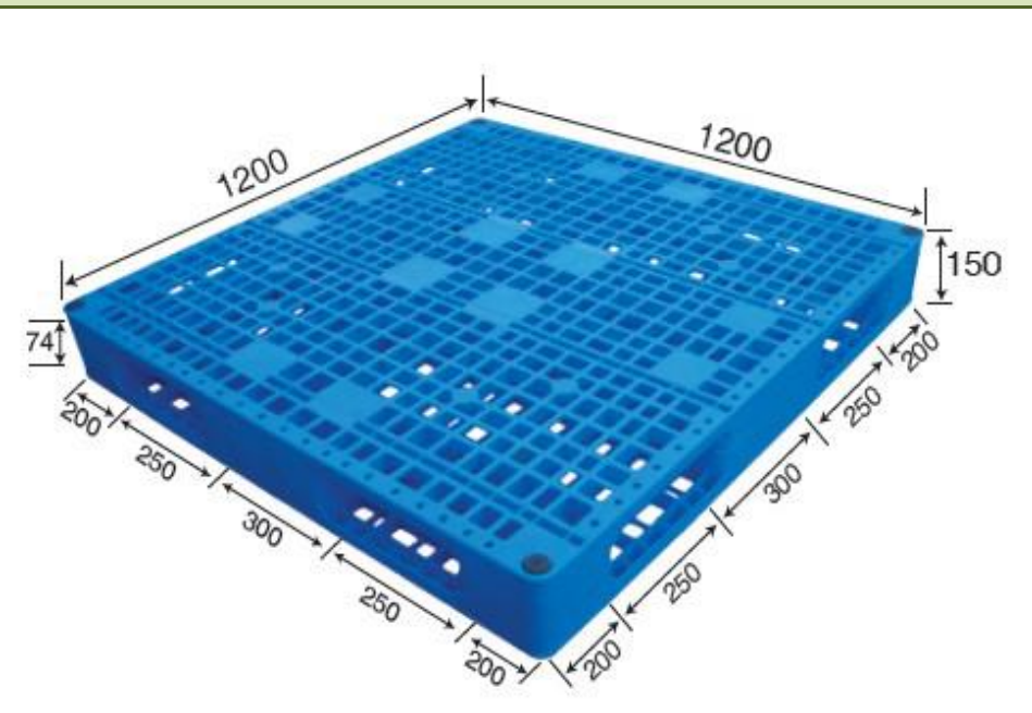
No. 394 MS - 1212D Reversible
