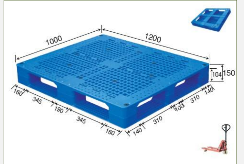
No. 122 MS - 1210E Double Deck
